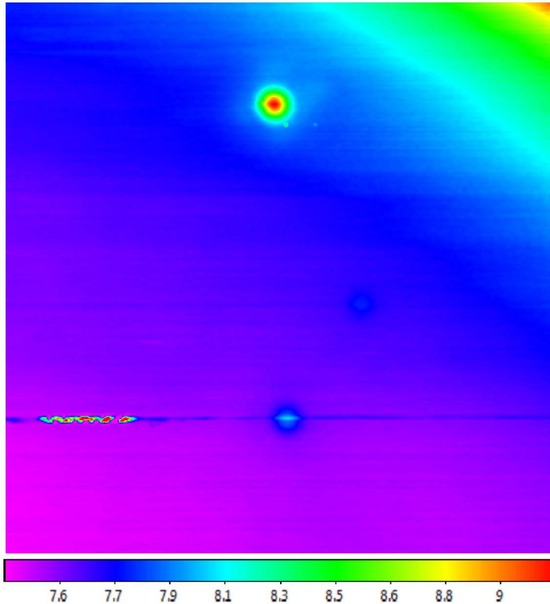
Figure 5. from Skynet Algorithm for Single-dish Radio Mapping. I. Contaminant-cleaning, Mapping, and Photometering Small-scale Structures null 2019 APJS 240 12 doi:10.3847/1538-4365/aad7c1 https://dx.doi.org/10.3847/1538-4365/aad7c1 © 2019. The American Astronomical Society. All rights reserved.
