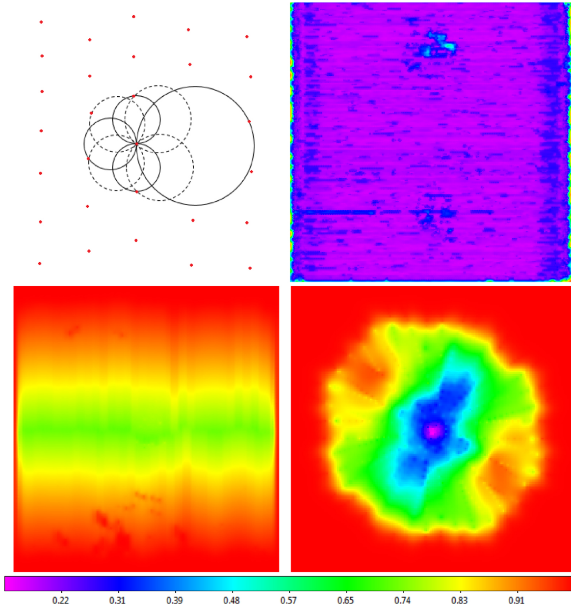
Figure 49. from Skynet Algorithm for Single-dish Radio Mapping. I. Contaminant-cleaning, Mapping, and Photometering Small-scale Structures null 2019 APJS 240 12 doi:10.3847/1538-4365/aad7c1 https://dx.doi.org/10.3847/1538-4365/aad7c1 © 2019. The American Astronomical Society. All rights reserved.
