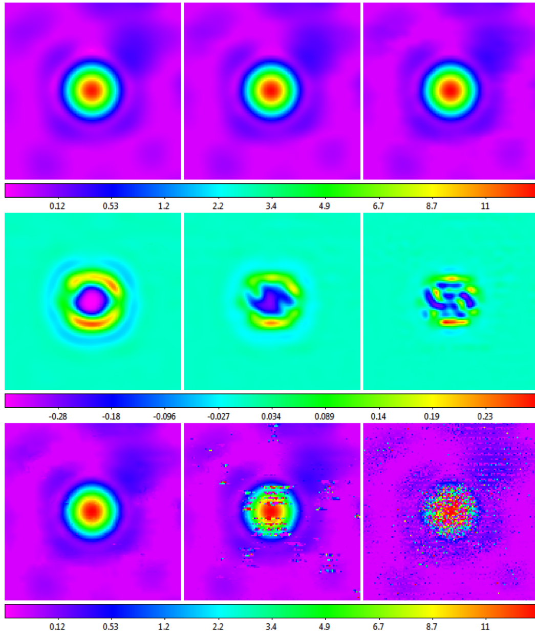
Figure 47. from Skynet Algorithm for Single-dish Radio Mapping. I. Contaminant-cleaning, Mapping, and Photometering Small-scale Structures null 2019 APJS 240 12 doi:10.3847/1538-4365/aad7c1 https://dx.doi.org/10.3847/1538-4365/aad7c1 © 2019. The American Astronomical Society. All rights reserved.
