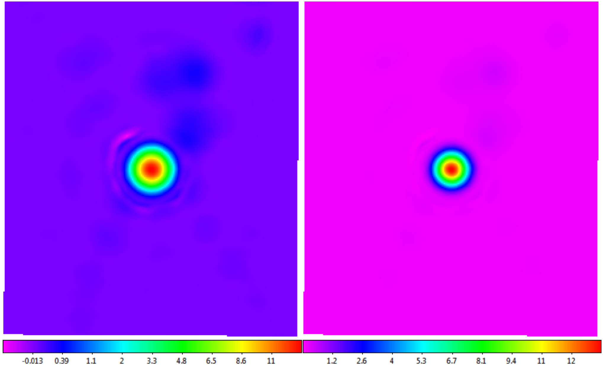
Figure 45. from Skynet Algorithm for Single-dish Radio Mapping. I. Contaminant-cleaning, Mapping, and Photometering Small-scale Structures null 2019 APJS 240 12 doi:10.3847/1538-4365/aad7c1 https://dx.doi.org/10.3847/1538-4365/aad7c1 © 2019. The American Astronomical Society. All rights reserved.
