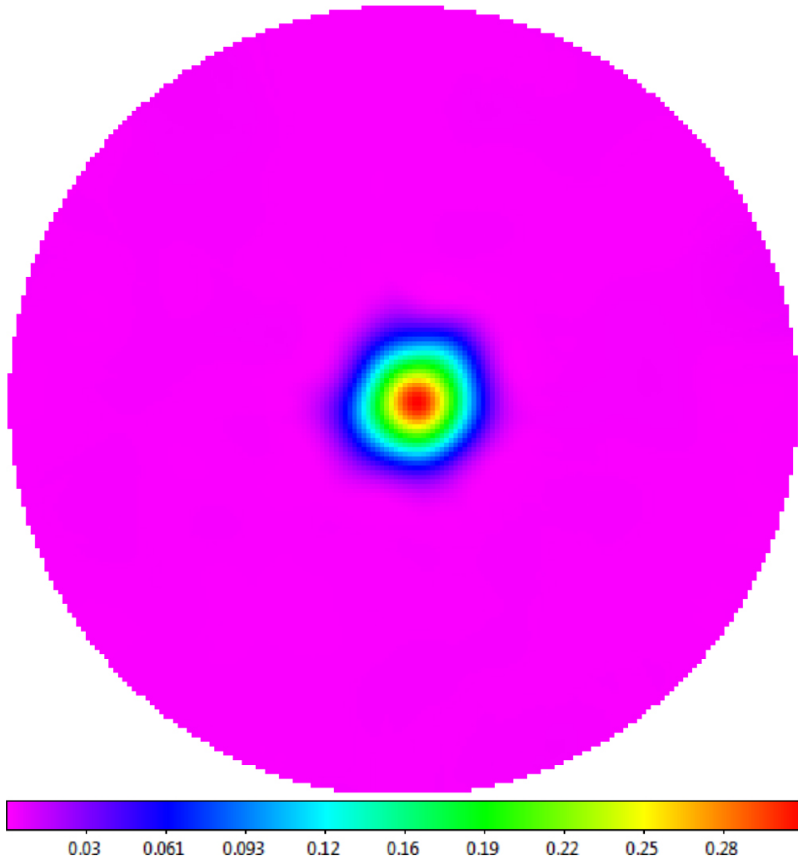
Figure 44. from Skynet Algorithm for Single-dish Radio Mapping. I. Contaminant-cleaning, Mapping, and Photometering Small-scale Structures null 2019 APJS 240 12 doi:10.3847/1538-4365/aad7c1 https://dx.doi.org/10.3847/1538-4365/aad7c1 © 2019. The American Astronomical Society. All rights reserved.
