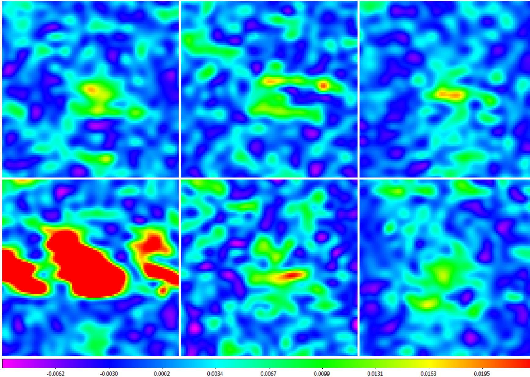
Figure 41. from Skynet Algorithm for Single-dish Radio Mapping. I. Contaminant-cleaning, Mapping, and Photometering Small-scale Structures null 2019 APJS 240 12 doi:10.3847/1538-4365/aad7c1 https://dx.doi.org/10.3847/1538-4365/aad7c1 © 2019. The American Astronomical Society. All rights reserved.
