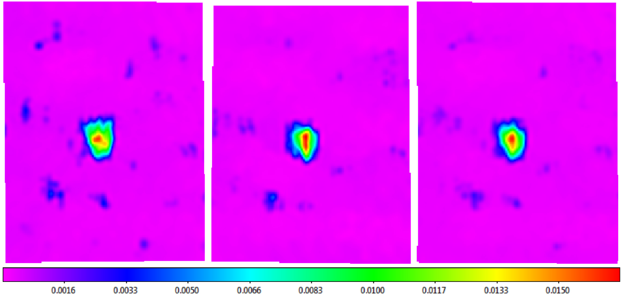
Figure 40. from Skynet Algorithm for Single-dish Radio Mapping. I. Contaminant-cleaning, Mapping, and Photometering Small-scale Structures null 2019 APJS 240 12 doi:10.3847/1538-4365/aad7c1 https://dx.doi.org/10.3847/1538-4365/aad7c1 © 2019. The American Astronomical Society. All rights reserved.
