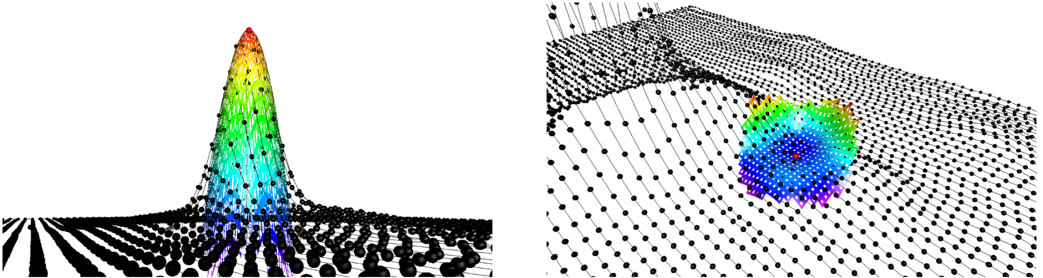
Figure 4. from Skynet Algorithm for Single-dish Radio Mapping. I. Contaminant-cleaning, Mapping, and Photometering Small-scale Structures null 2019 APJS 240 12 doi:10.3847/1538-4365/aad7c1 https://dx.doi.org/10.3847/1538-4365/aad7c1 © 2019. The American Astronomical Society. All rights reserved.
