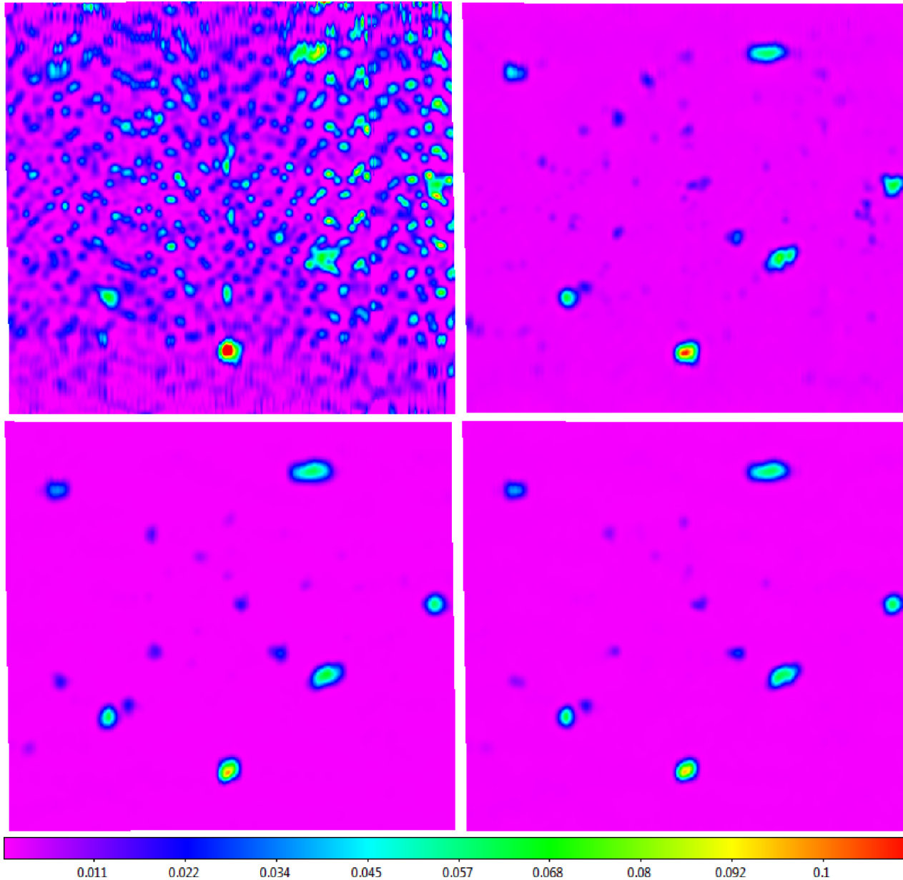
Figure 39. from Skynet Algorithm for Single-dish Radio Mapping. I. Contaminant-cleaning, Mapping, and Photometering Small-scale Structures null 2019 APJS 240 12 doi:10.3847/1538-4365/aad7c1 https://dx.doi.org/10.3847/1538-4365/aad7c1 © 2019. The American Astronomical Society. All rights reserved.
