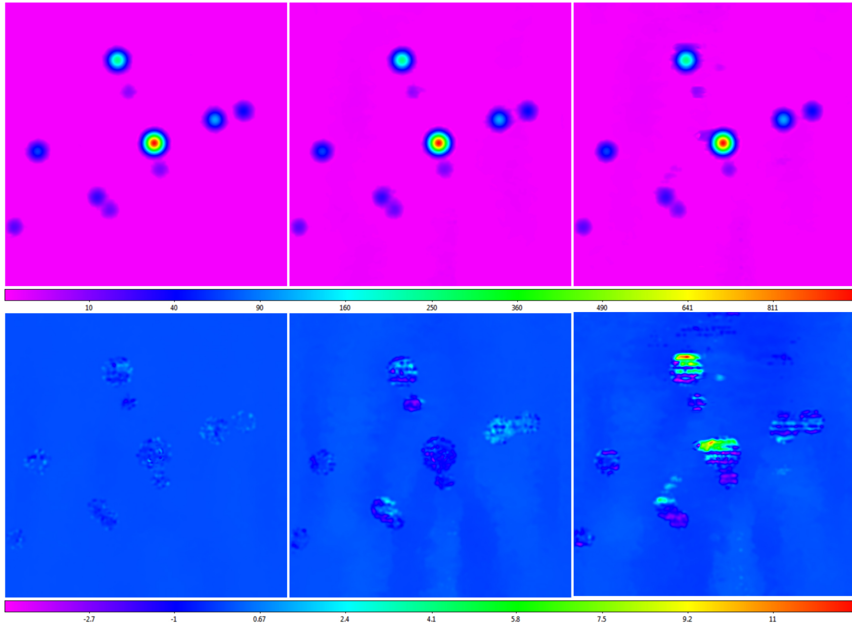
Figure 37. from Skynet Algorithm for Single-dish Radio Mapping. I. Contaminant-cleaning, Mapping, and Photometry Small-scale Structures null 2019 APJS 240 12 doi:10.3847/1538-4365/aad7c1 https://dx.doi.org/10.3847/1538-4365/aad7c1 © 2019. The American Astronomical Society. All rights reserved.
