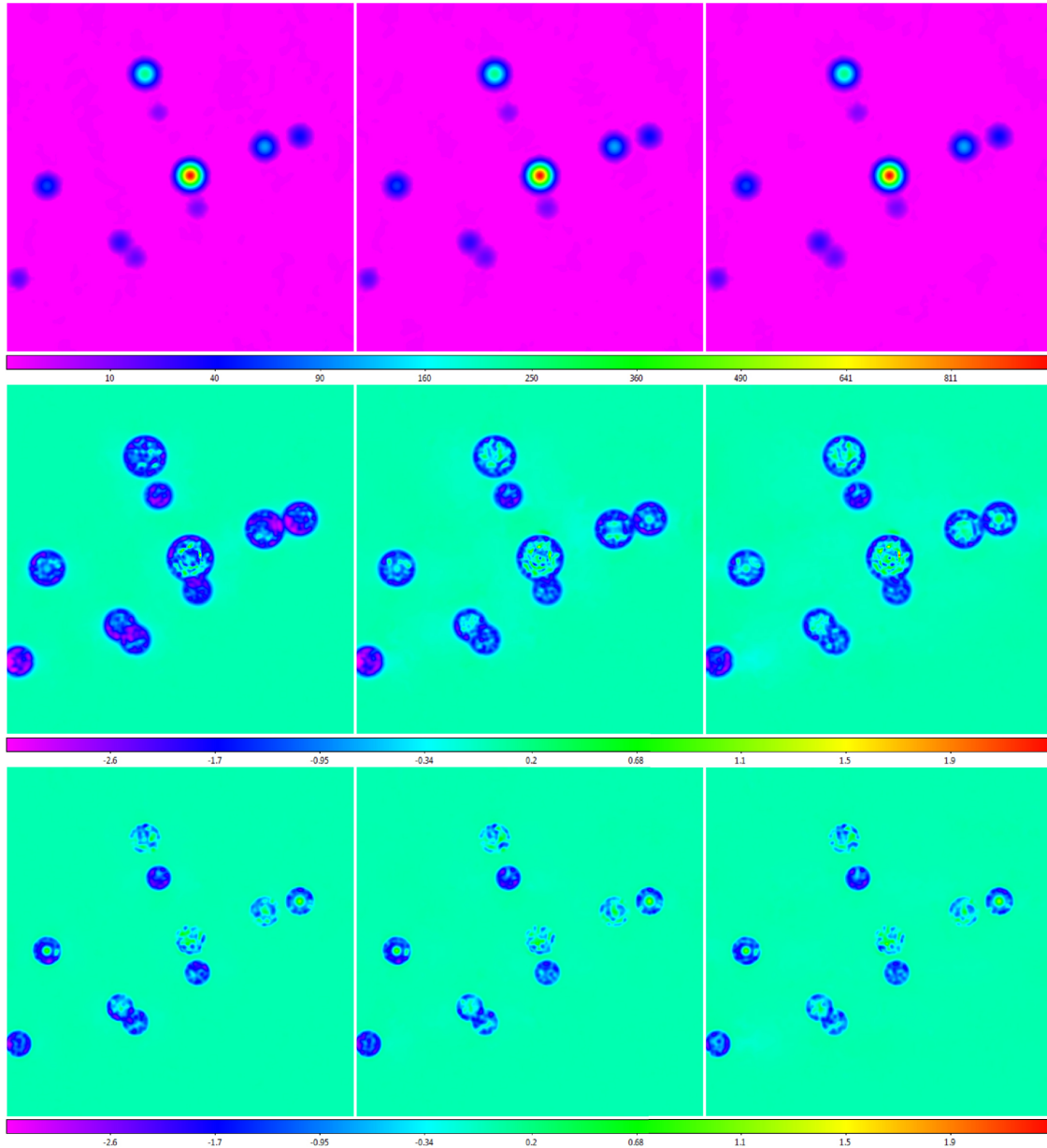
Figure 35. from Skynet Algorithm for Single-dish Radio Mapping. I. Contaminant-cleaning, Mapping, and Photometering Small-scale Structures null 2019 APJS 240 12 doi:10.3847/1538-4365/aad7c1 https://dx.doi.org/10.3847/1538-4365/aad7c1 © 2019. The American Astronomical Society. All rights reserved.
