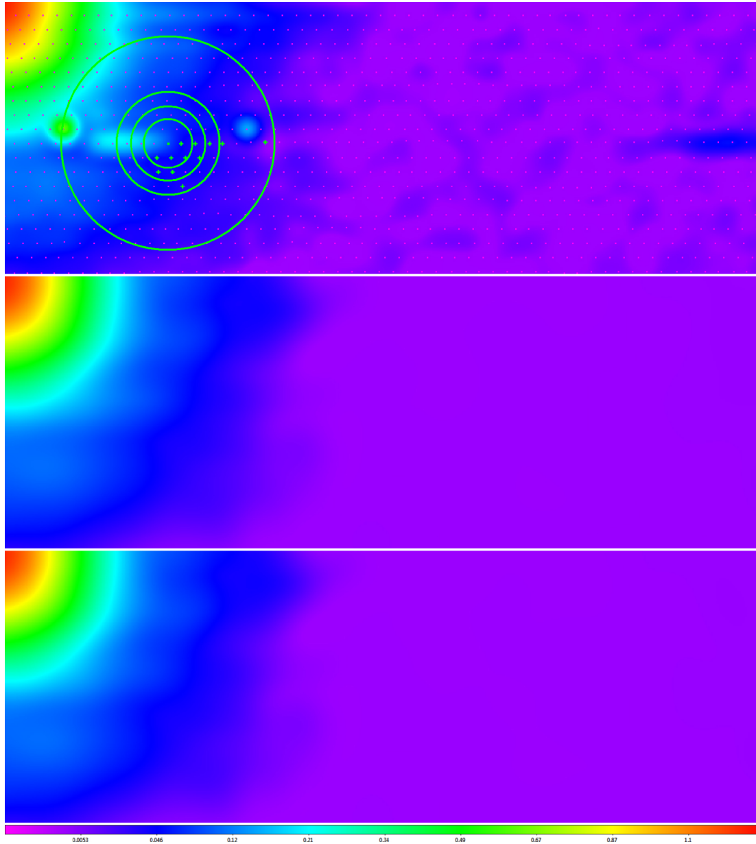
Figure 33. from Skynet Algorithm for Single-dish Radio Mapping. I. Contaminant-cleaning, Mapping, and Photometering Small-scale Structures null 2019 APJS 240 12 doi:10.3847/1538-4365/aad7c1 https://dx.doi.org/10.3847/1538-4365/aad7c1 © 2019. The American Astronomical Society. All rights reserved.
