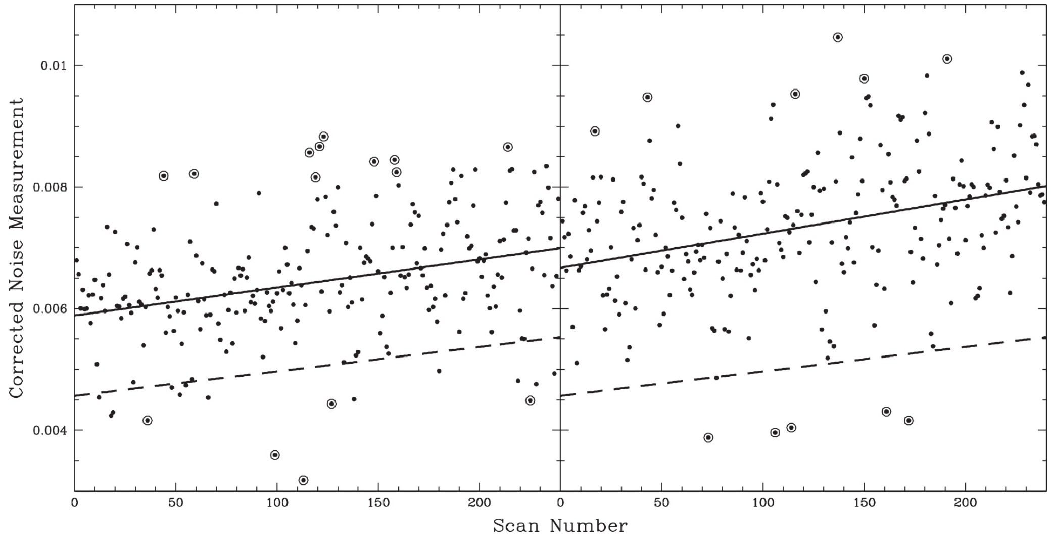
Figure 30. from Skynet Algorithm for Single-dish Radio Mapping. I. Contaminant-cleaning, Mapping, and Photometering Small-scale Structures null 2019 APJS 240 12 doi:10.3847/1538-4365/aad7c1 https://dx.doi.org/10.3847/1538-4365/aad7c1 © 2019. The American Astronomical Society. All rights reserved.
