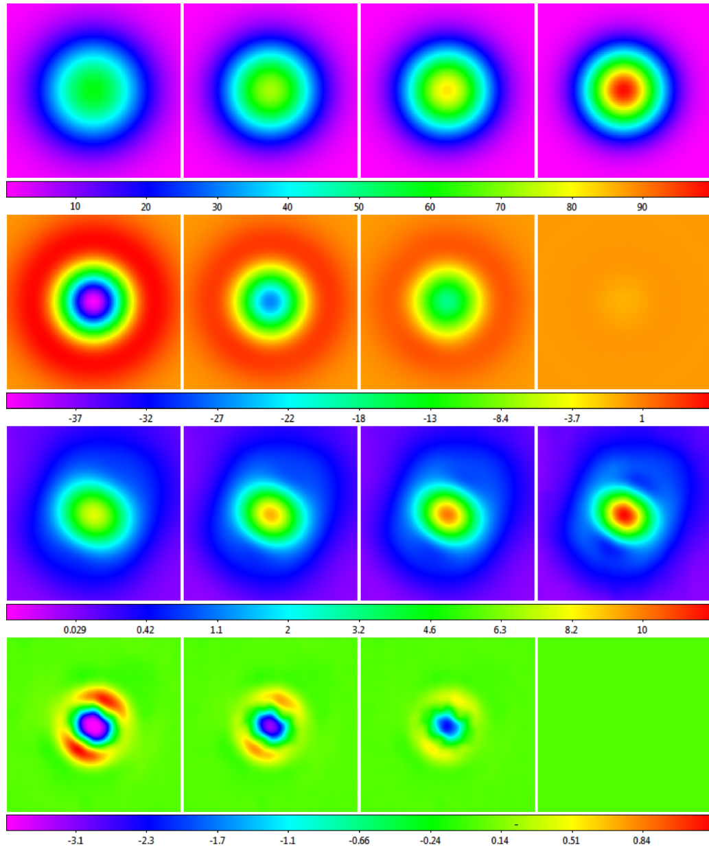
Figure 3. from Skynet Algorithm for Single-dish Radio Mapping. I. Contaminant-cleaning, Mapping, and Photometering Small-scale Structures null 2019 APJS 240 12 doi:10.3847/1538-4365/aad7c1 https://dx.doi.org/10.3847/1538-4365/aad7c1 © 2019. The American Astronomical Society. All rights reserved.
