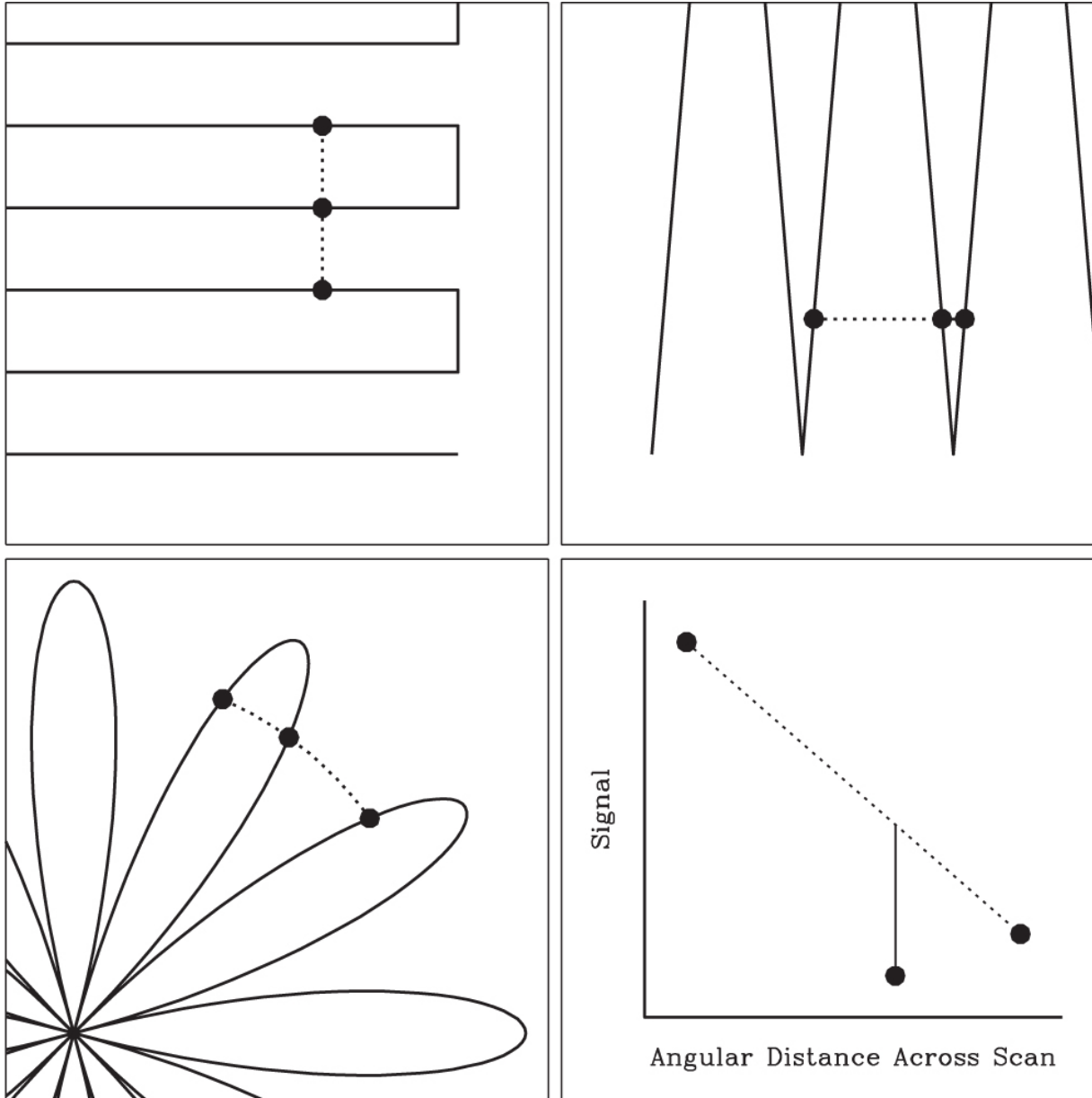
Figure 29. from Skynet Algorithm for Single-dish Radio Mapping. I. Contaminant-cleaning, Mapping, and Photometering Small-scale Structures null 2019 APJS 240 12 doi:10.3847/1538-4365/aad7c1 https://dx.doi.org/10.3847/1538-4365/aad7c1 © 2019. The American Astronomical Society. All rights reserved.
