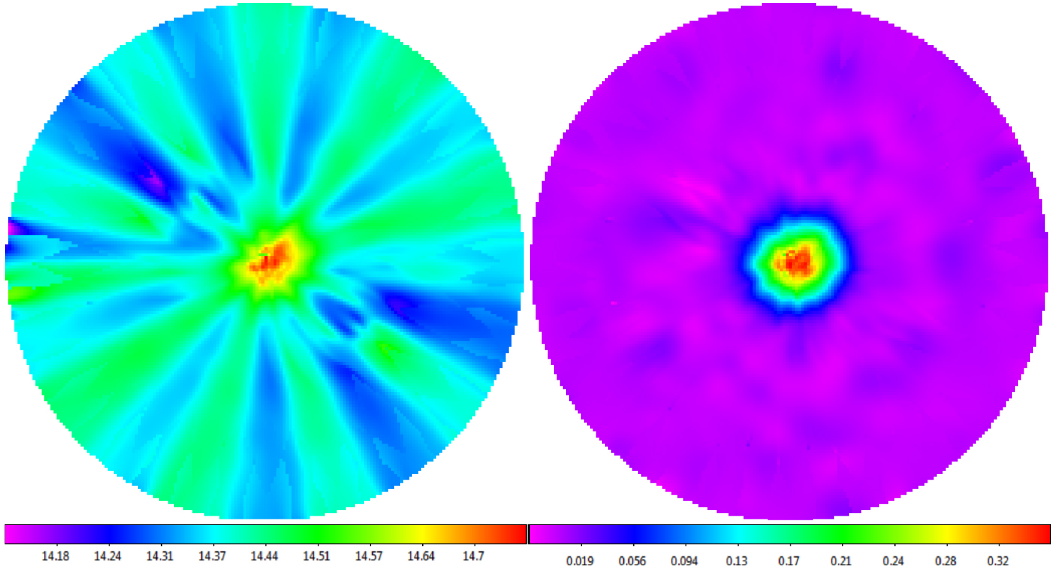
Figure 25. from Skynet Algorithm for Single-dish Radio Mapping. I. Contaminant-cleaning, Mapping, and Photometering Small-scale Structures null 2019 APJS 240 12 doi:10.3847/1538-4365/aad7c1 https://dx.doi.org/10.3847/1538-4365/aad7c1 © 2019. The American Astronomical Society. All rights reserved.
