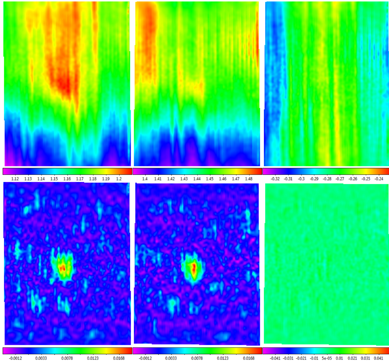
Figure 24. from Skynet Algorithm for Single-dish Radio Mapping. I. Contaminant-cleaning, Mapping, and Photometering Small-scale Structures null 2019 APJS 240 12 doi:10.3847/1538-4365/aad7c1 https://dx.doi.org/10.3847/1538-4365/aad7c1 © 2019. The American Astronomical Society. All rights reserved.
