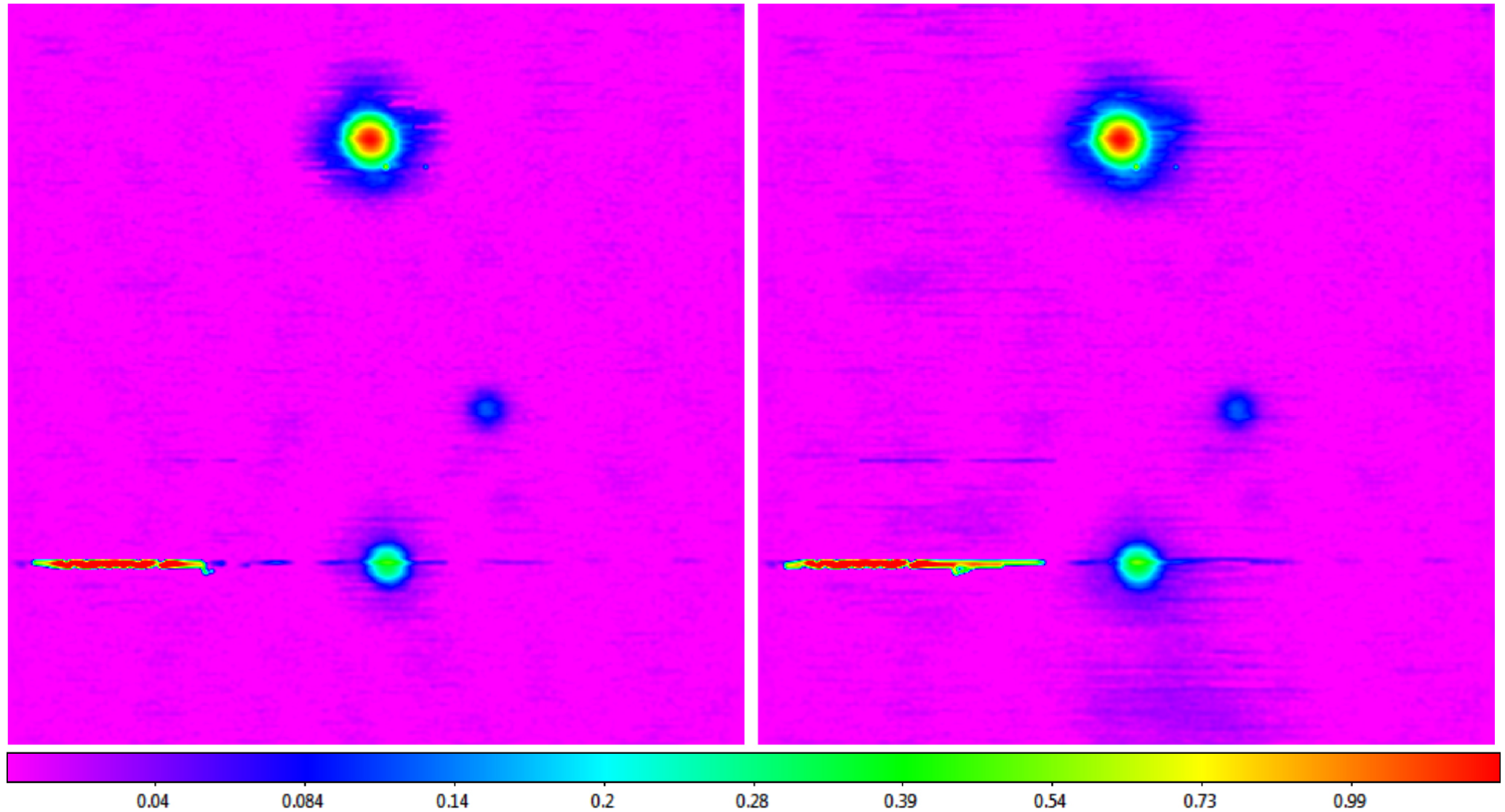
Figure 23. from Skynet Algorithm for Single-dish Radio Mapping. I. Contaminant-cleaning, Mapping, and Photometering Small-scale Structures null 2019 APJS 240 12 doi:10.3847/1538-4365/aad7c1 https://dx.doi.org/10.3847/1538-4365/aad7c1 © 2019. The American Astronomical Society. All rights reserved.
