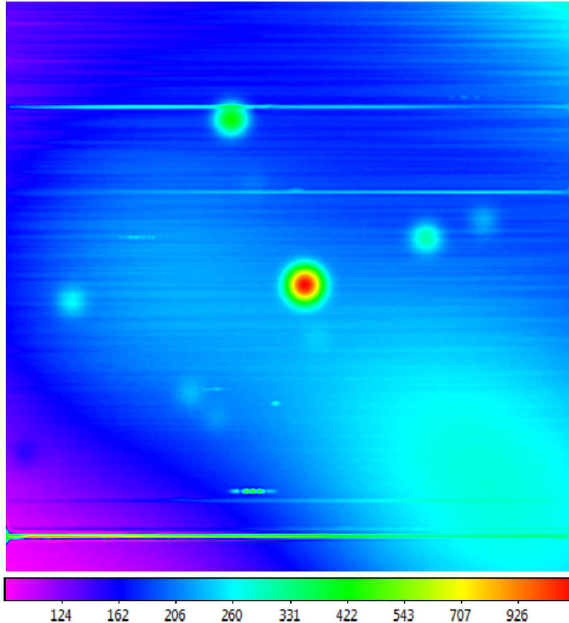
Figure 21. from Skynet Algorithm for Single-dish Radio Mapping. I. Contaminant-cleaning, Mapping, and Photometering Small-scale Structures null 2019 APJS 240 12 doi:10.3847/1538-4365/aad7c1 https://dx.doi.org/10.3847/1538-4365/aad7c1 © 2019. The American Astronomical Society. All rights reserved.
