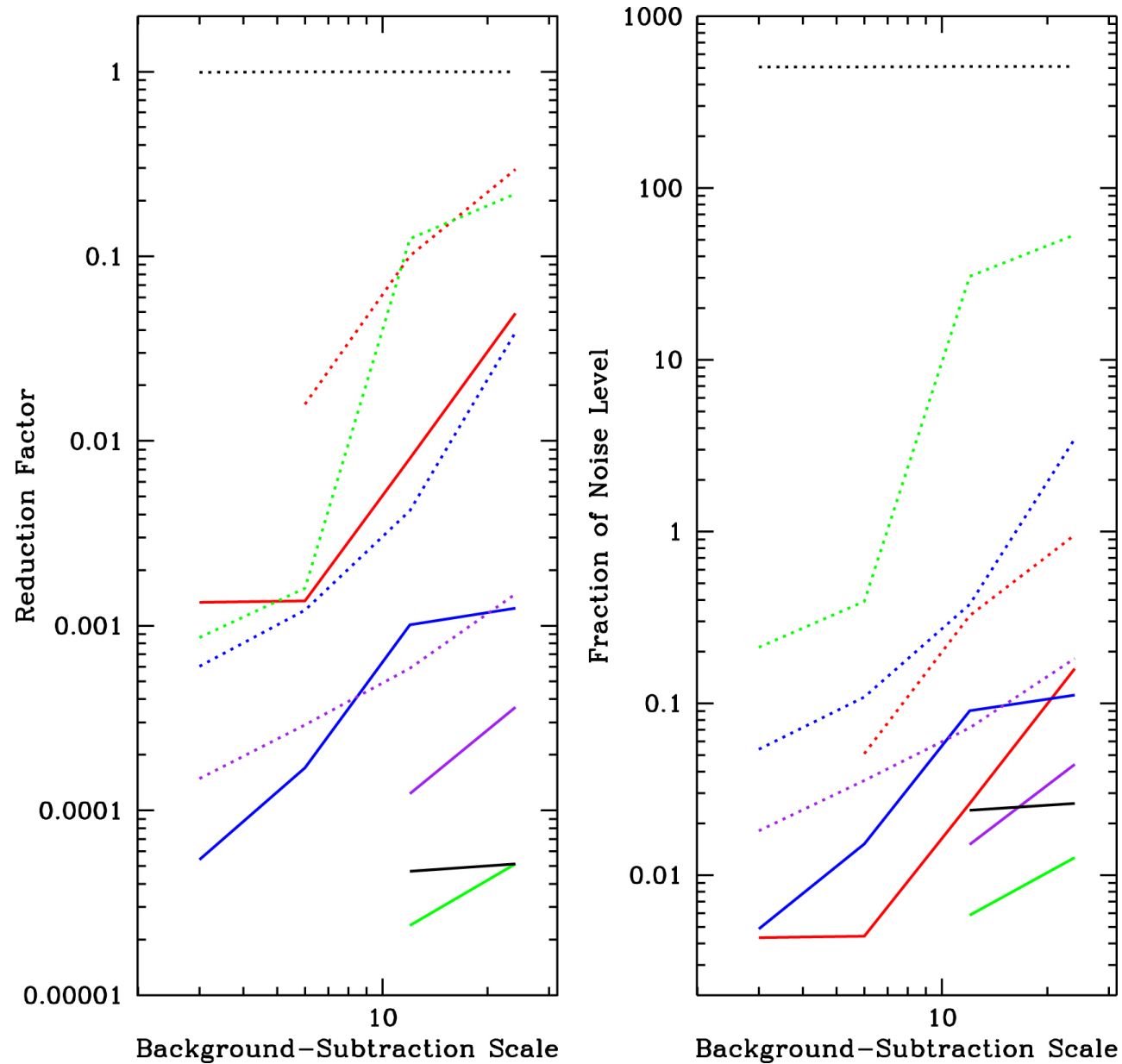
Figure 20. from Skynet Algorithm for Single-dish Radio Mapping. I. Contaminant-cleaning, Mapping, and Photometering Small-scale Structures null 2019 APJS 240 12 doi:10.3847/1538-4365/aad7c1 https://dx.doi.org/10.3847/1538-4365/aad7c1 © 2019. The American Astronomical Society. All rights reserved.
