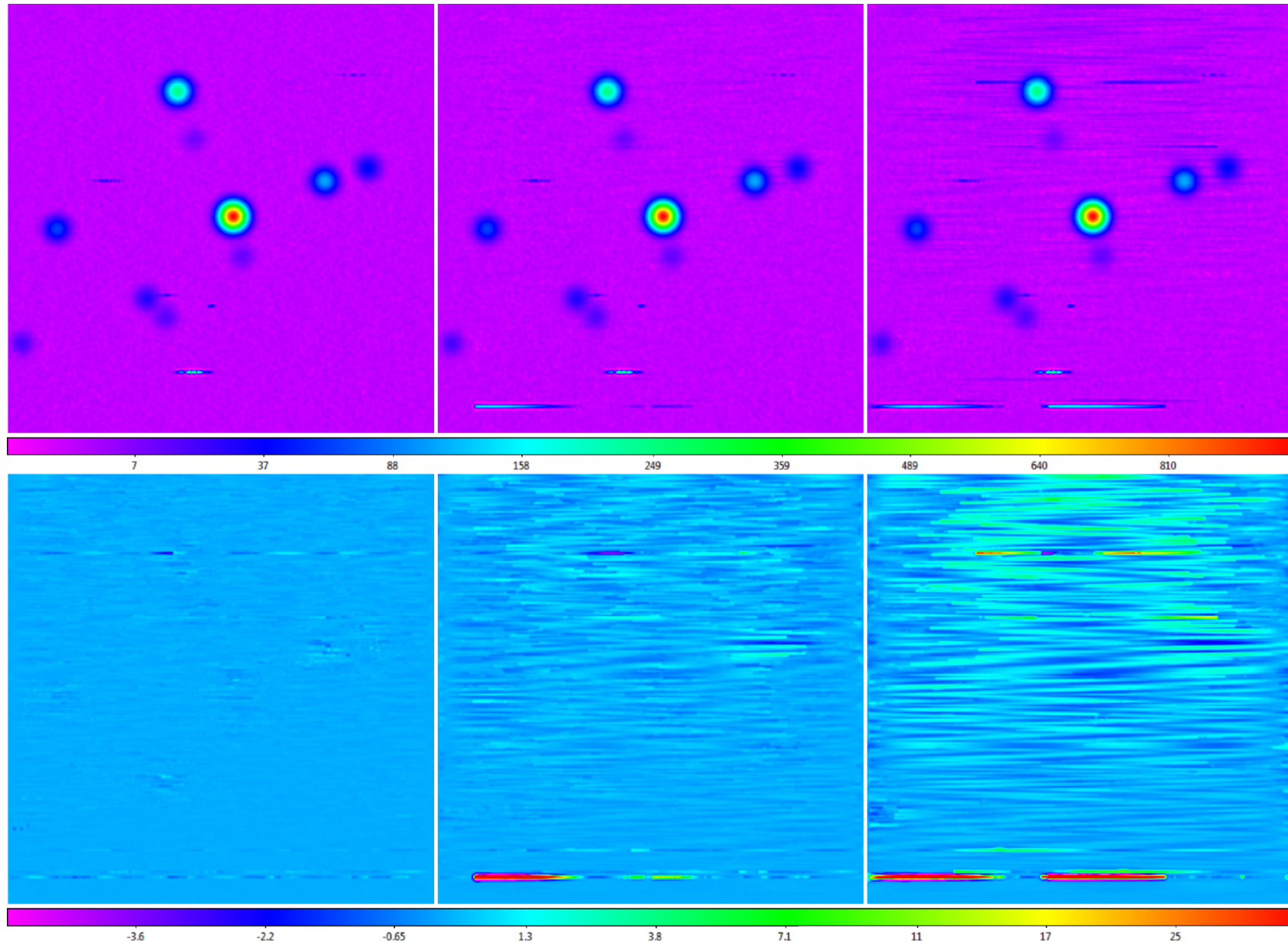
Figure 19. from Skynet Algorithm for Single-dish Radio Mapping. I. Contaminant-cleaning, Mapping, and Photometering Small-scale Structures null 2019 APJS 240 12 doi:10.3847/1538-4365/aad7c1 https://dx.doi.org/10.3847/1538-4365/aad7c1 © 2019. The American Astronomical Society. All rights reserved.
