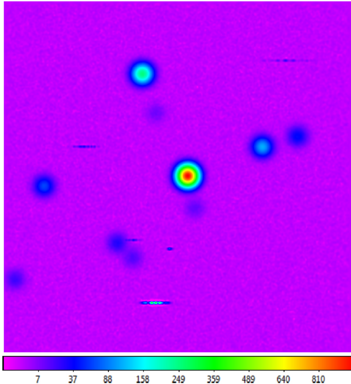
Figure 16. from Skynet Algorithm for Single-dish Radio Mapping. I. Contaminant-cleaning, Mapping, and Photometering Small-scale Structures null 2019 APJS 240 12 doi:10.3847/1538-4365/aad7c1 https://dx.doi.org/10.3847/1538-4365/aad7c1 © 2019. The American Astronomical Society. All rights reserved.
