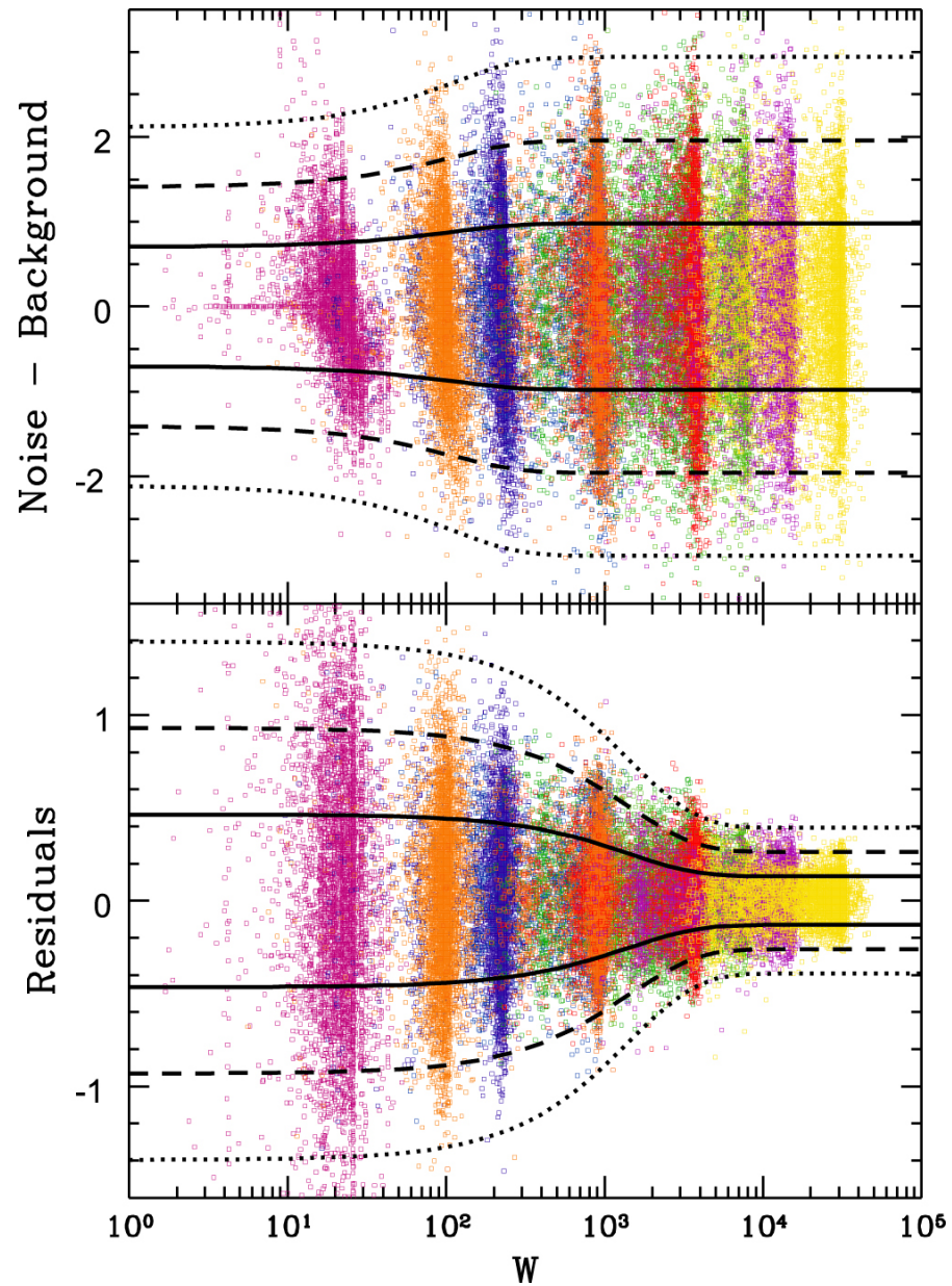
Figure 15. from Skynet Algorithm for Single-dish Radio Mapping. I. Contaminant-cleaning, Mapping, and Photometering Small-scale Structures null 2019 APJS 240 12 doi:10.3847/1538-4365/aad7c1 https://dx.doi.org/10.3847/1538-4365/aad7c1 © 2019. The American Astronomical Society. All rights reserved.
