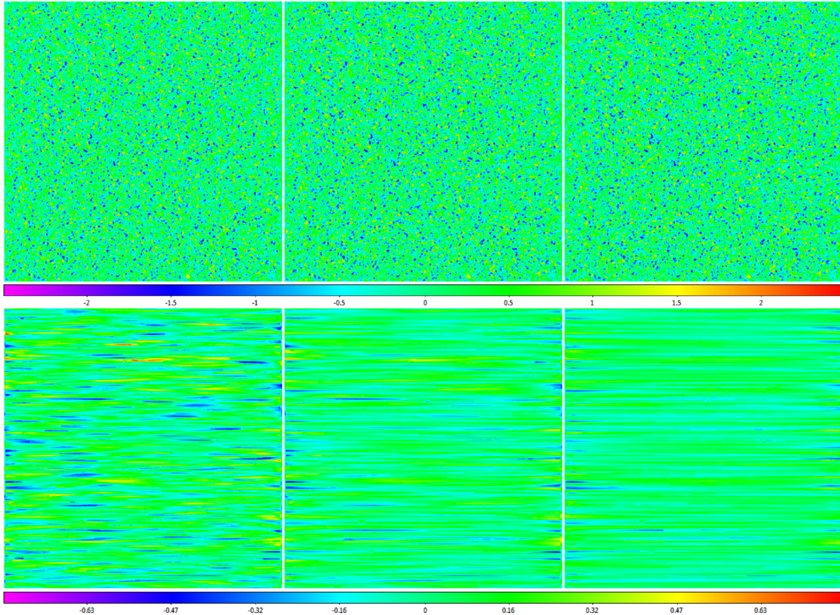
Figure 14. from Skynet Algorithm for Single-dish Radio Mapping. I. Contaminant-cleaning, Mapping, and Photometering Small-scale Structures null 2019 APJS 240 12 doi:10.3847/1538-4365/aad7c1 https://dx.doi.org/10.3847/1538-4365/aad7c1 © 2019. The American Astronomical Society. All rights reserved.
