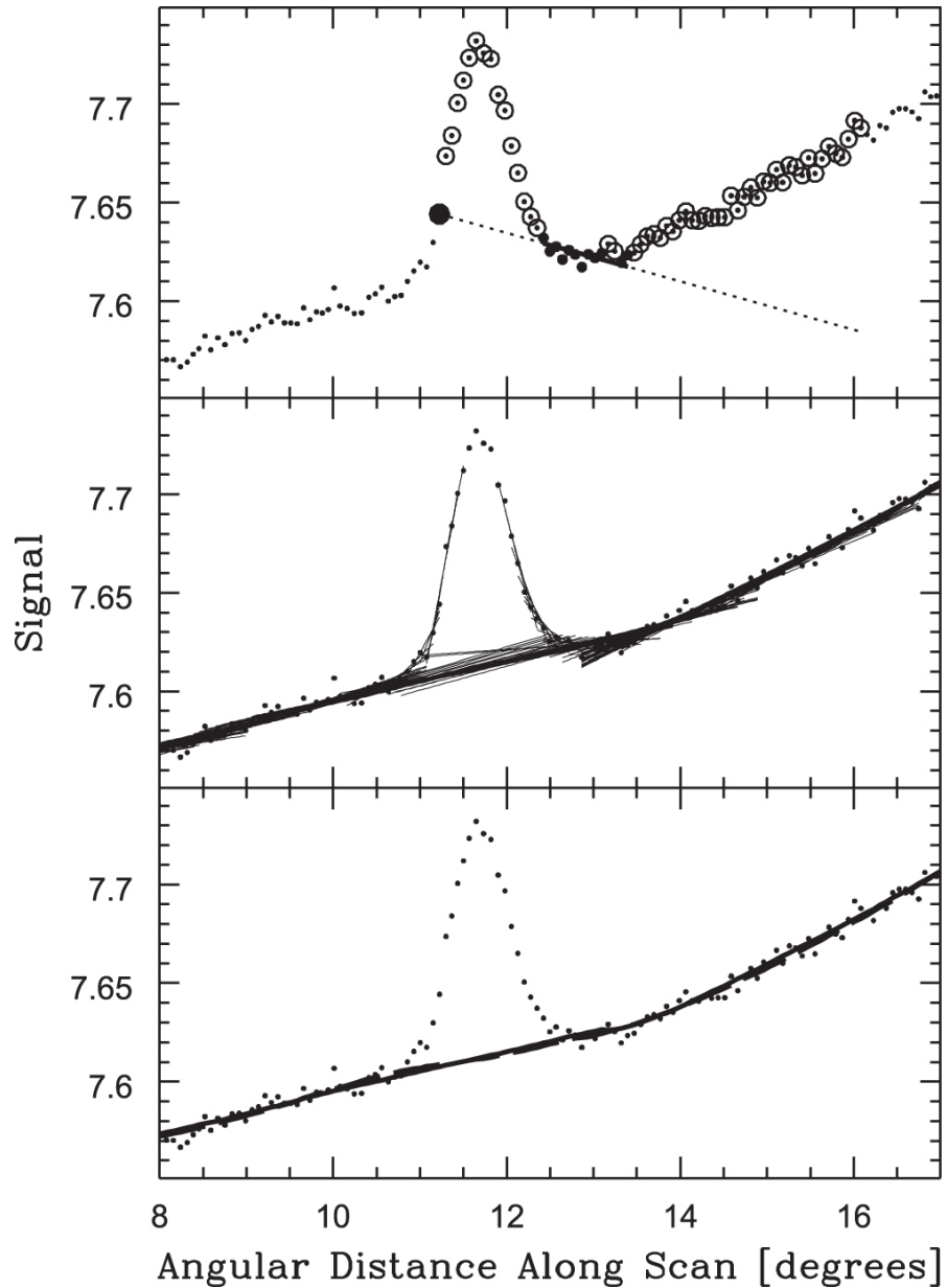
Figure 12. from Skynet Algorithm for Single-dish Radio Mapping. I. Contaminant-cleaning, Mapping, and Photometering Small-scale Structures null 2019 APJS 240 12 doi:10.3847/1538-4365/aad7c1 https://dx.doi.org/10.3847/1538-4365/aad7c1 © 2019. The American Astronomical Society. All rights reserved.
