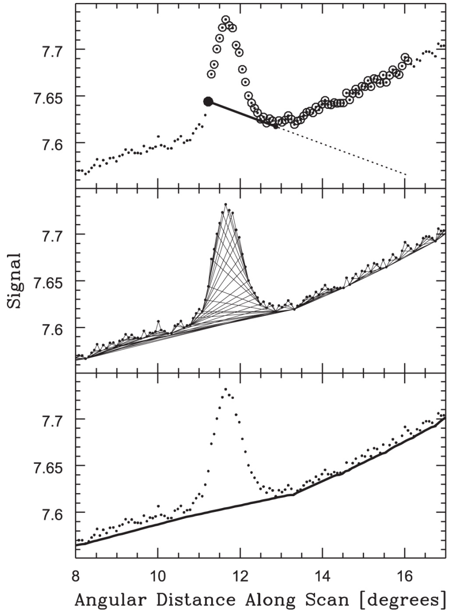
Figure 11. from Skynet Algorithm for Single-dish Radio Mapping. I. Contaminant-cleaning, Mapping, and Photometering Small-scale Structures null 2019 APJS 240 12 doi:10.3847/1538-4365/aad7c1 https://dx.doi.org/10.3847/1538-4365/aad7c1 © 2019. The American Astronomical Society. All rights reserved.
