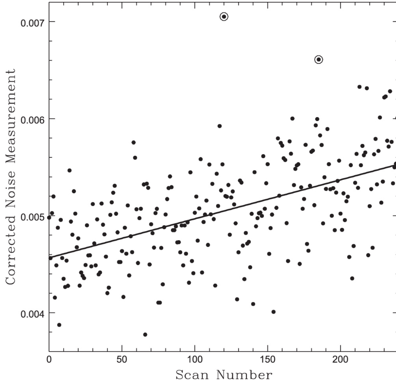
Figure 10. from Skynet Algorithm for Single-dish Radio Mapping. I. Contaminant-cleaning, Mapping, and Photometering Small-scale Structures null 2019 APJS 240 12 doi:10.3847/1538-4365/aad7c1 https://dx.doi.org/10.3847/1538-4365/aad7c1 © 2019. The American Astronomical Society. All rights reserved.
