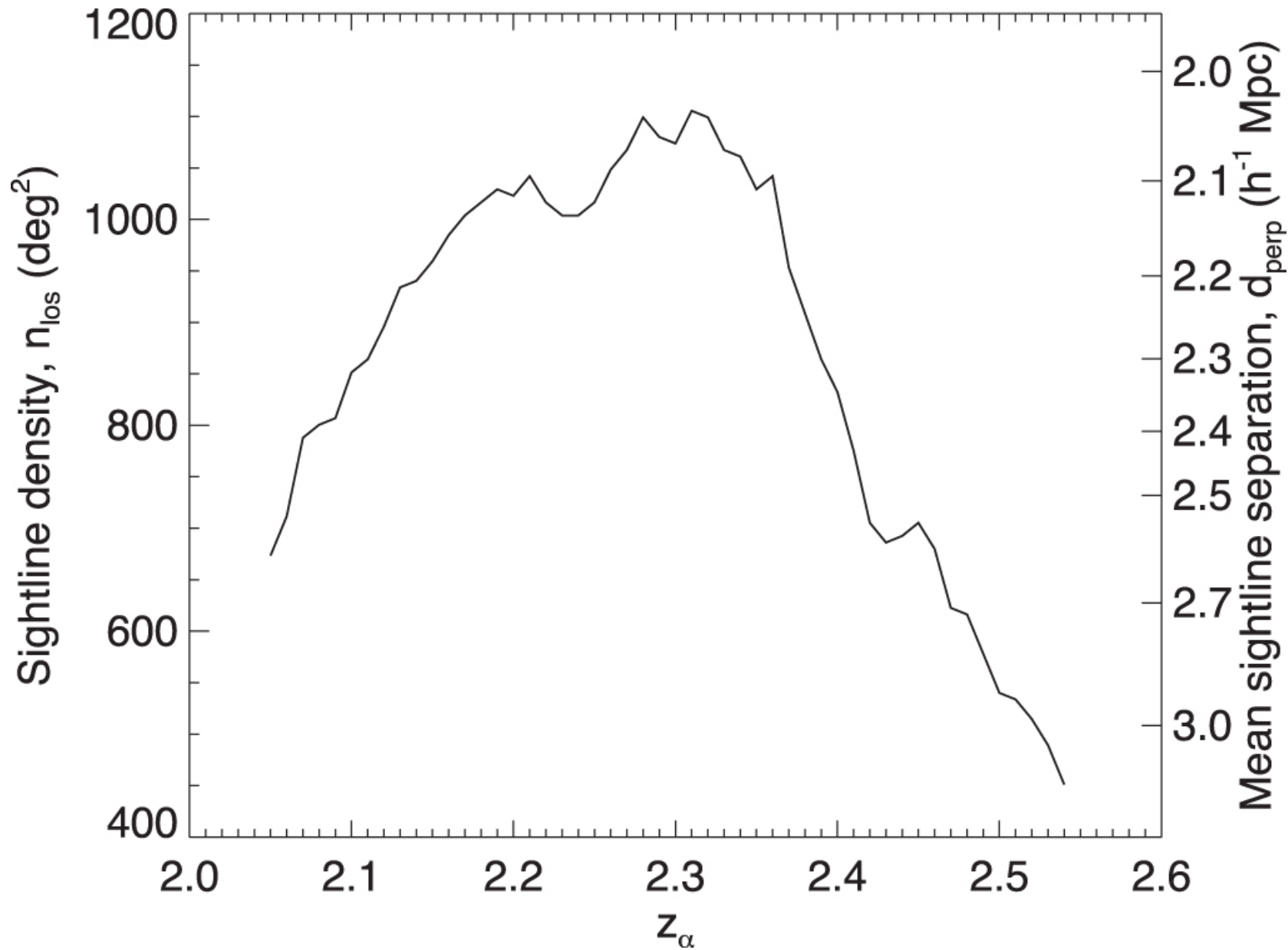
Figure 8. from First Data Release of the COSMOS Ly Mapping and Tomography Observations: 3D Ly Forest Tomography at 2.05 < z < 2.55 null 2018 APJS 237 31 doi:10.3847/1538-4365/aace58 https://dx.doi.org/10.3847/1538-4365/aace58 © 2018. The American Astronomical Society. All rights reserved.
