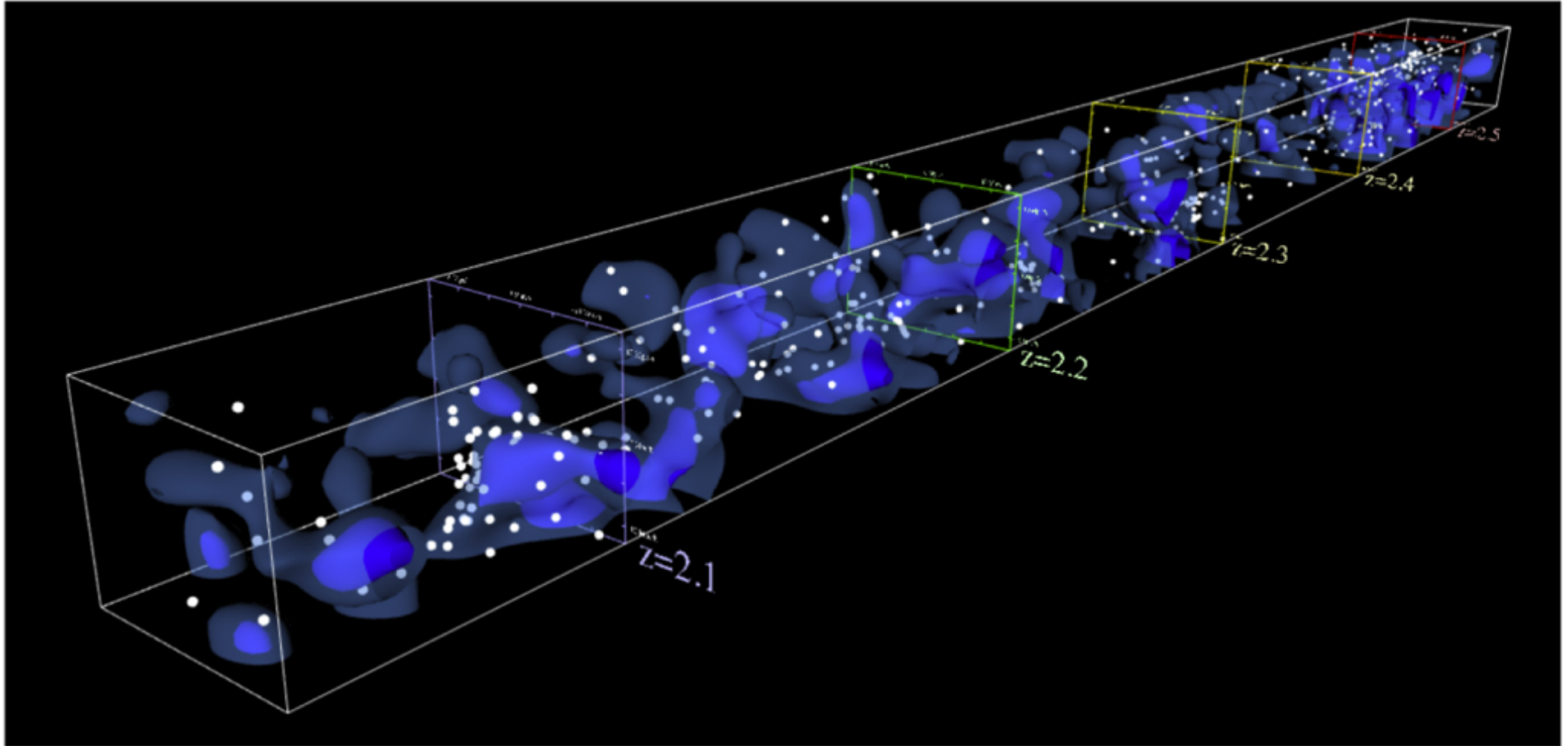
Figure 11. from First Data Release of the COSMOS Ly Mapping and Tomography Observations: 3D Ly Forest Tomography at 2.05 < z < 2.55 null 2018 APJS 237 31 doi:10.3847/1538-4365/aace58 https://dx.doi.org/10.3847/1538-4365/aace58 © 2018. The American Astronomical Society. All rights reserved.
