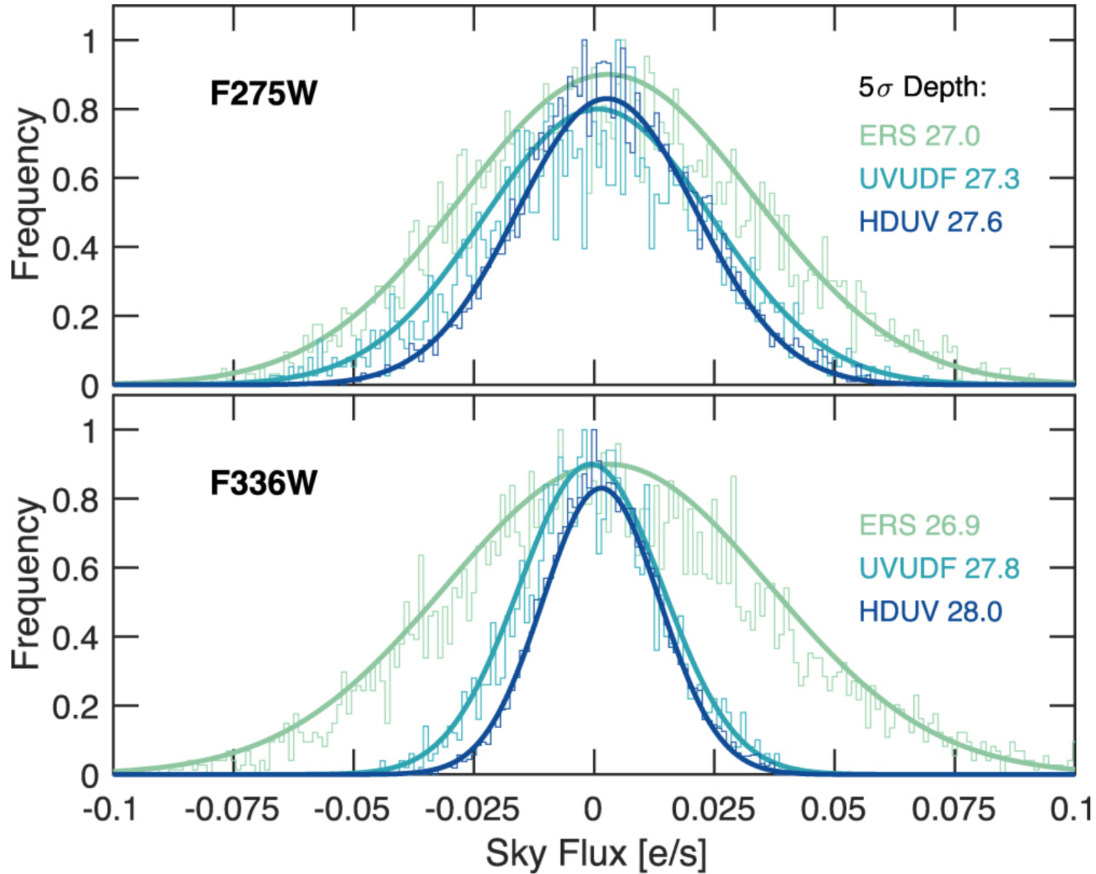
Figure 8. from HDUV: The Hubble Deep UV Legacy Survey null 2018 APJS 237 12 doi:10.3847/1538-4365/aacb30 https://dx.doi.org/10.3847/1538-4365/aacb30 © 2018. The American Astronomical Society. All rights reserved.
