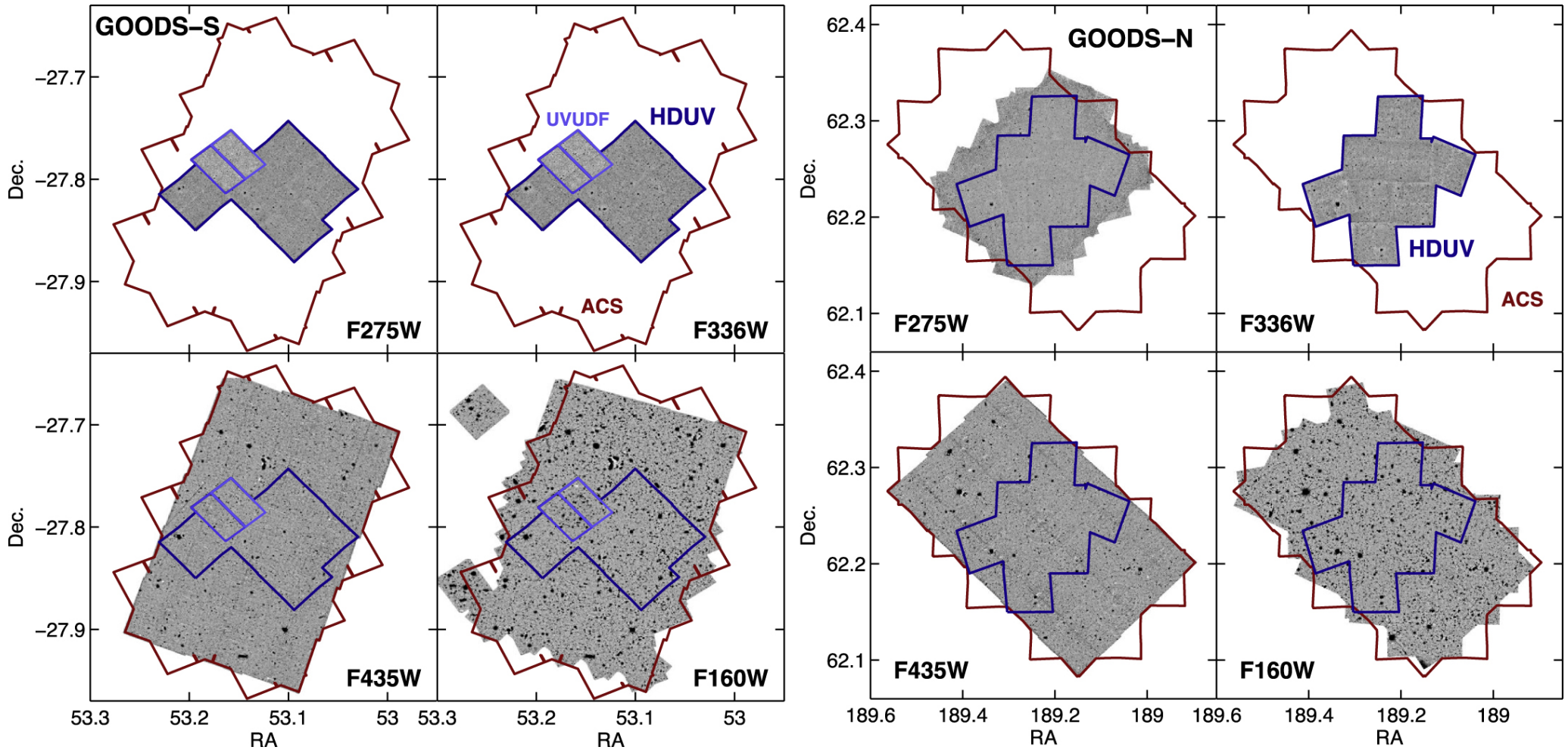
Figure 6. from HDUV: The Hubble Deep UV Legacy Survey null 2018 APJS 237 12 doi:10.3847/1538-4365/aacb30 https://dx.doi.org/10.3847/1538-4365/aacb30 © 2018. The American Astronomical Society. All rights reserved.
