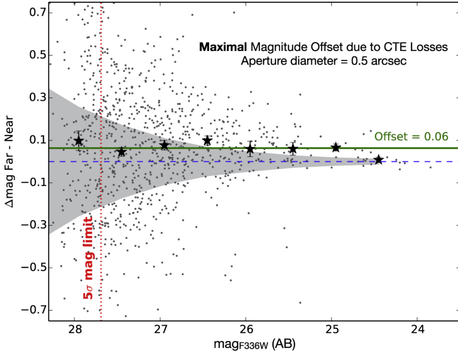
Figure 3. from HDUV: The Hubble Deep UV Legacy Survey null 2018 APJS 237 12 doi:10.3847/1538-4365/aacb30 https://dx.doi.org/10.3847/1538-4365/aacb30 © 2018. The American Astronomical Society. All rights reserved.
