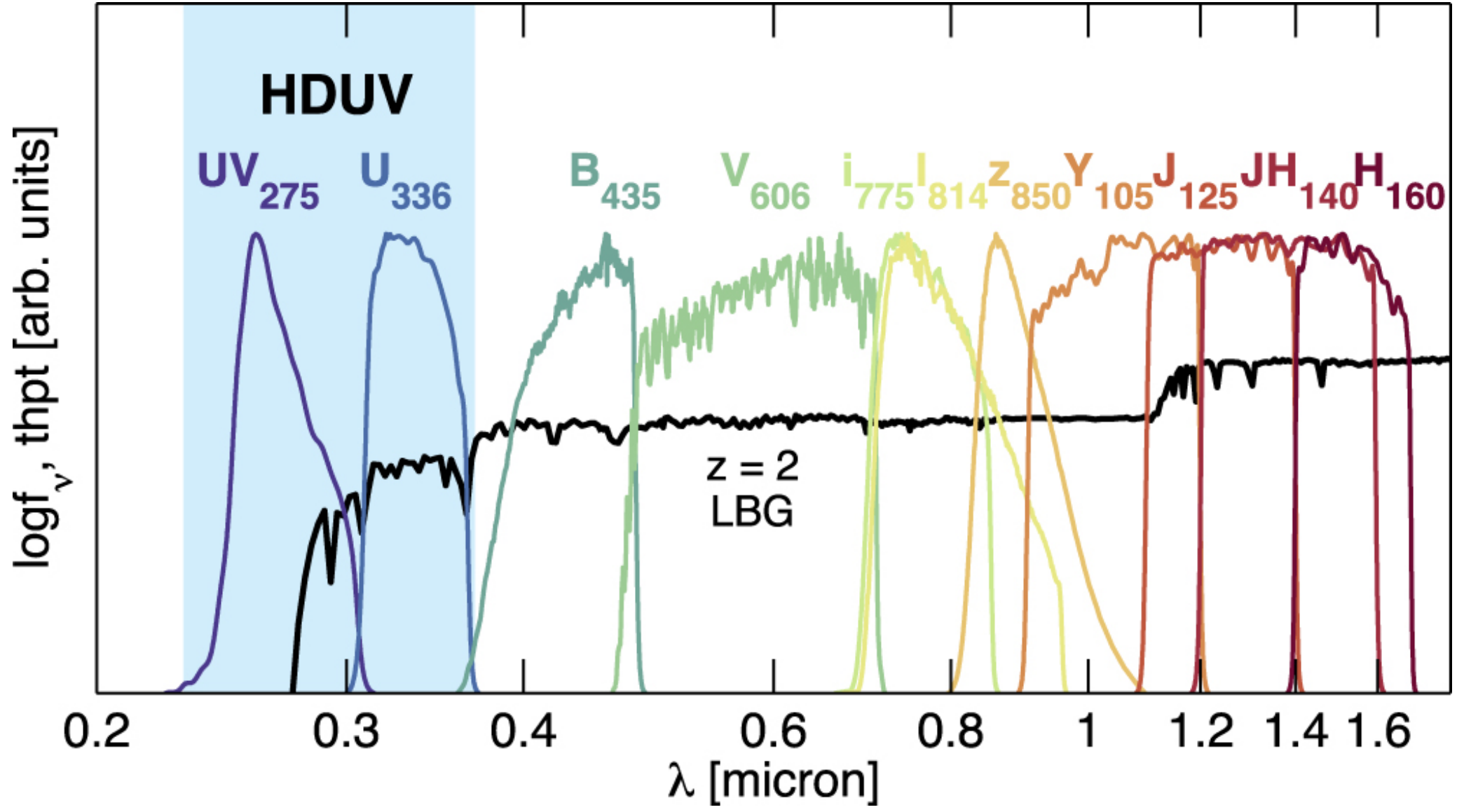
Figure 2. from HDUV: The Hubble Deep UV Legacy Survey null 2018 APJS 237 12 doi:10.3847/1538-4365/aacb30 https://dx.doi.org/10.3847/1538-4365/aacb30 © 2018. The American Astronomical Society. All rights reserved.
