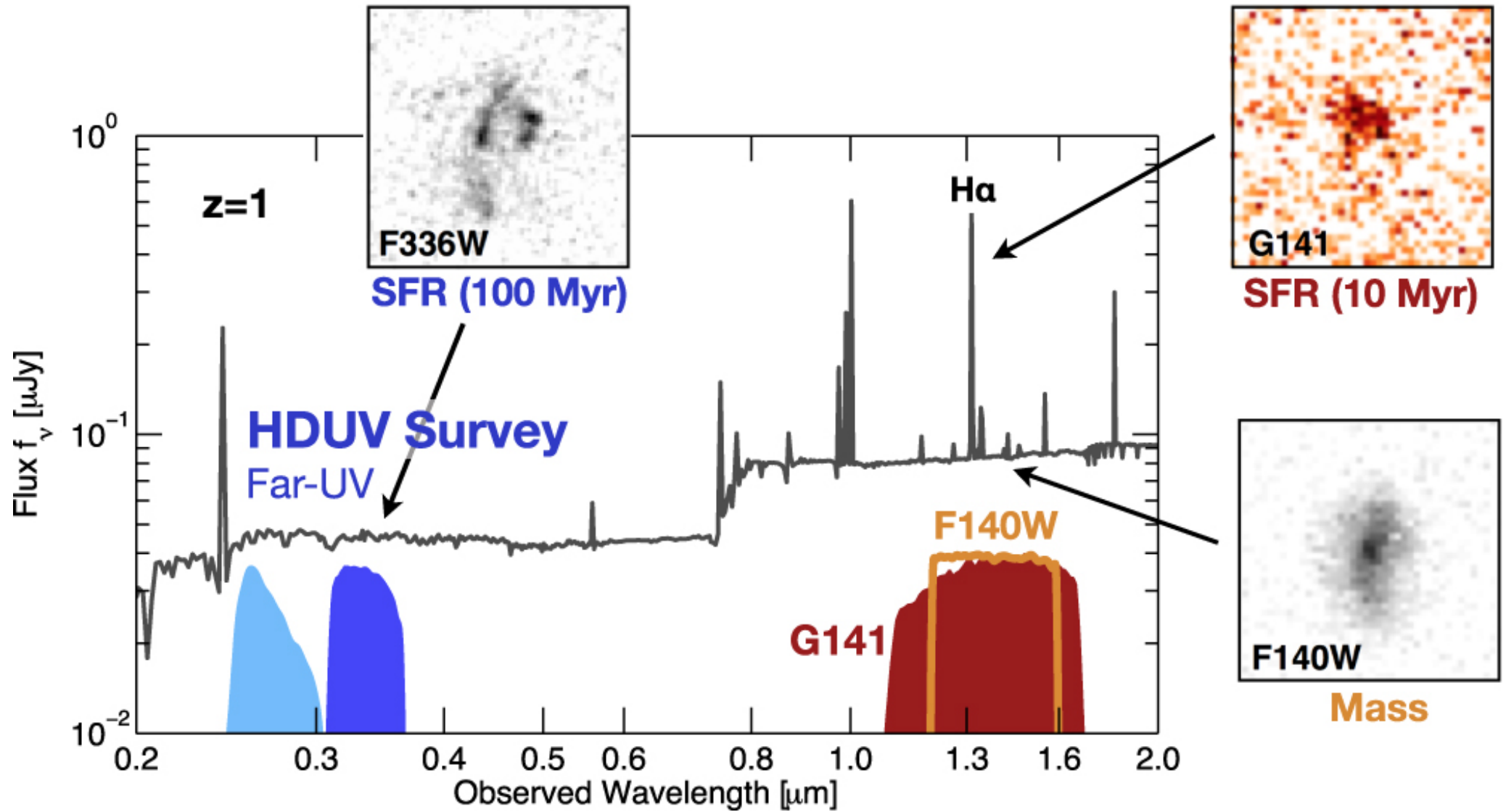
Figure 11. from HDUV: The Hubble Deep UV Legacy Survey null 2018 APJS 237 12 doi:10.3847/1538-4365/aacb30 https://dx.doi.org/10.3847/1538-4365/aacb30 © 2018. The American Astronomical Society. All rights reserved.
