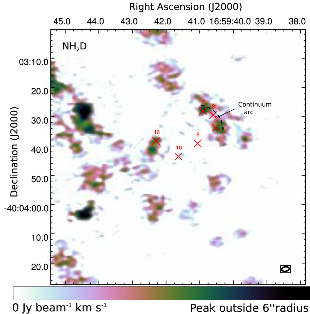
Figure 6. from Chemistry of the High-mass Protostellar Molecular Clump IRAS 16562–3959 null 2018 APJS 236 45 doi:10.3847/1538-4365/aac01d https://dx.doi.org/10.3847/1538-4365/aac01d © 2018. The American Astronomical Society. All rights reserved.
