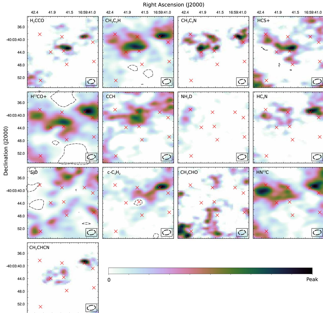
Figure 3. from Chemistry of the High-mass Protostellar Molecular Clump IRAS 16562–3959 null 2018 APJS 236 45 doi:10.3847/1538-4365/aac01d https://dx.doi.org/10.3847/1538-4365/aac01d © 2018. The American Astronomical Society. All rights reserved.
