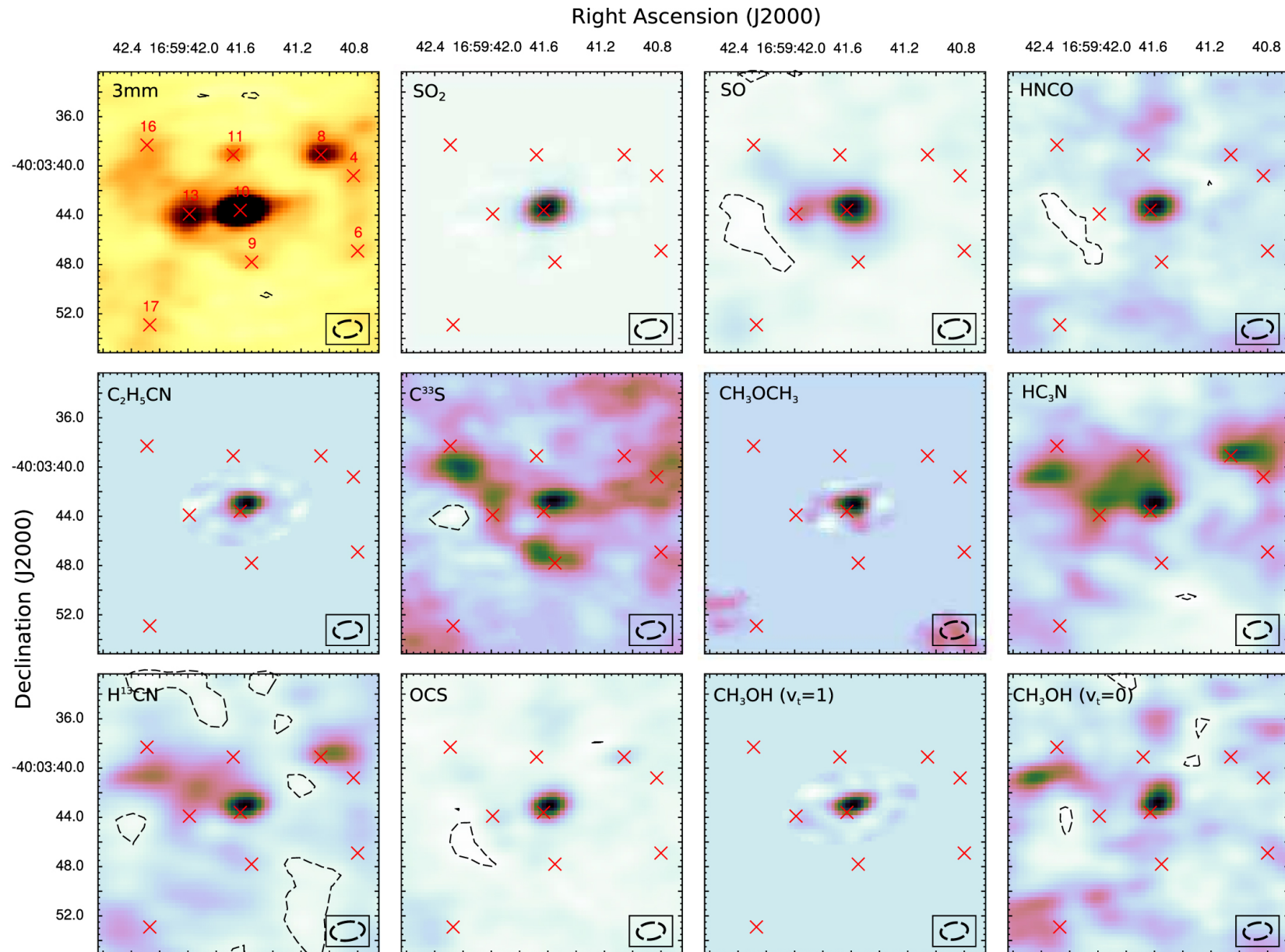
Figure 2. from Chemistry of the High-mass Protostellar Molecular Clump IRAS 16562–3959 null 2018 APJS 236 45 doi:10.3847/1538-4365/aac01d https://dx.doi.org/10.3847/1538-4365/aac01d © 2018. The American Astronomical Society. All rights reserved.
