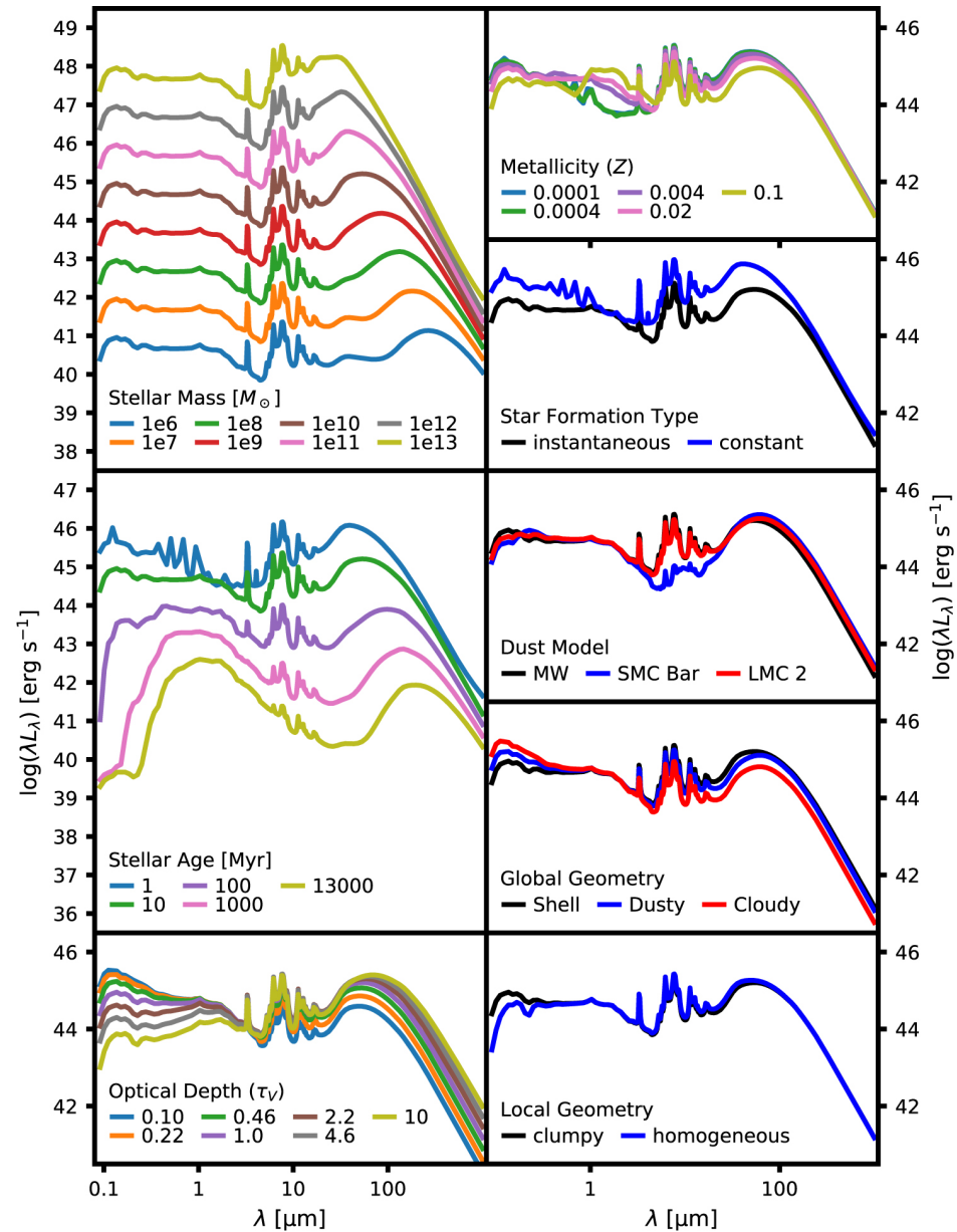
Figure 9. from DirtyGrid I: 3D Dust Radiative Transfer Modeling of Spectral Energy Distributions of Dusty Stellar Populations null 2018 APJS 236 32 doi:10.3847/1538-4365/aabf41 https://dx.doi.org/10.3847/1538-4365/aabf41
