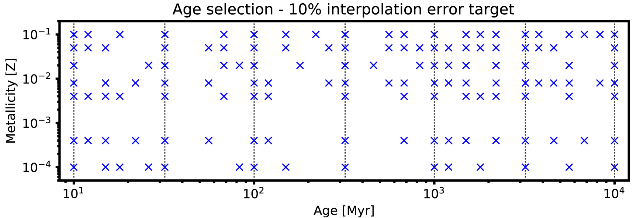
Figure 8. from DirtyGrid I: 3D Dust Radiative Transfer Modeling of Spectral Energy Distributions of Dusty Stellar Populations null 2018 APJS 236 32 doi:10.3847/1538-4365/aabf41 https://dx.doi.org/10.3847/1538-4365/aabf41 © 2018. The American Astronomical Society. All rights reserved.
