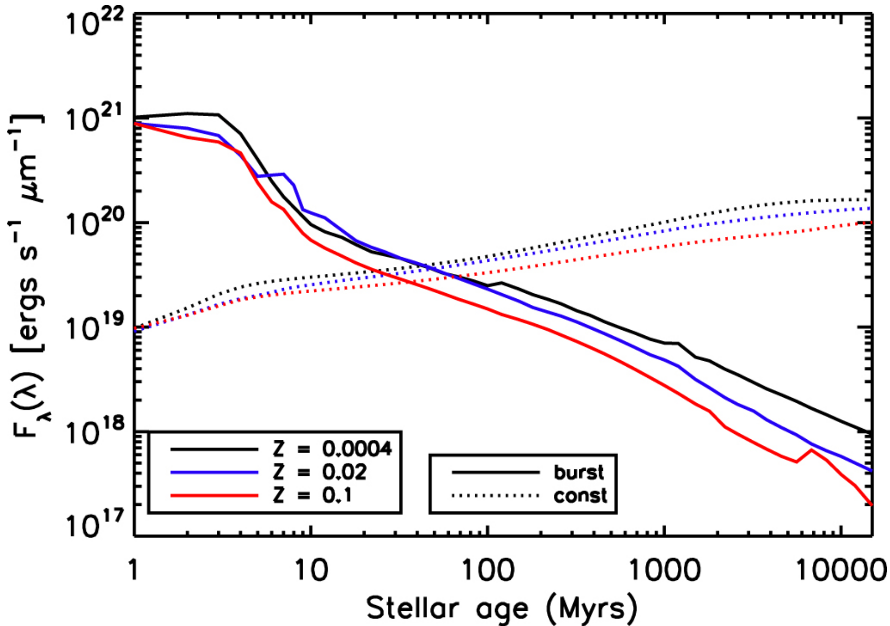
Figure 7. from DirtyGrid I: 3D Dust Radiative Transfer Modeling of Spectral Energy Distributions of Dusty Stellar Populations null 2018 APJS 236 32 doi:10.3847/1538-4365/aabf41 https://dx.doi.org/10.3847/1538-4365/aabf41 © 2018. The American Astronomical Society. All rights reserved.
