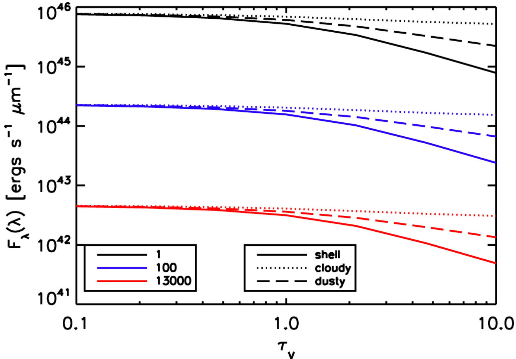
Figure 6. from DirtyGrid I: 3D Dust Radiative Transfer Modeling of Spectral Energy Distributions of Dusty Stellar Populations null 2018 APJS 236 32 doi:10.3847/1538-4365/aabf41 https://dx.doi.org/10.3847/1538-4365/aabf41 © 2018. The American Astronomical Society. All rights reserved.
