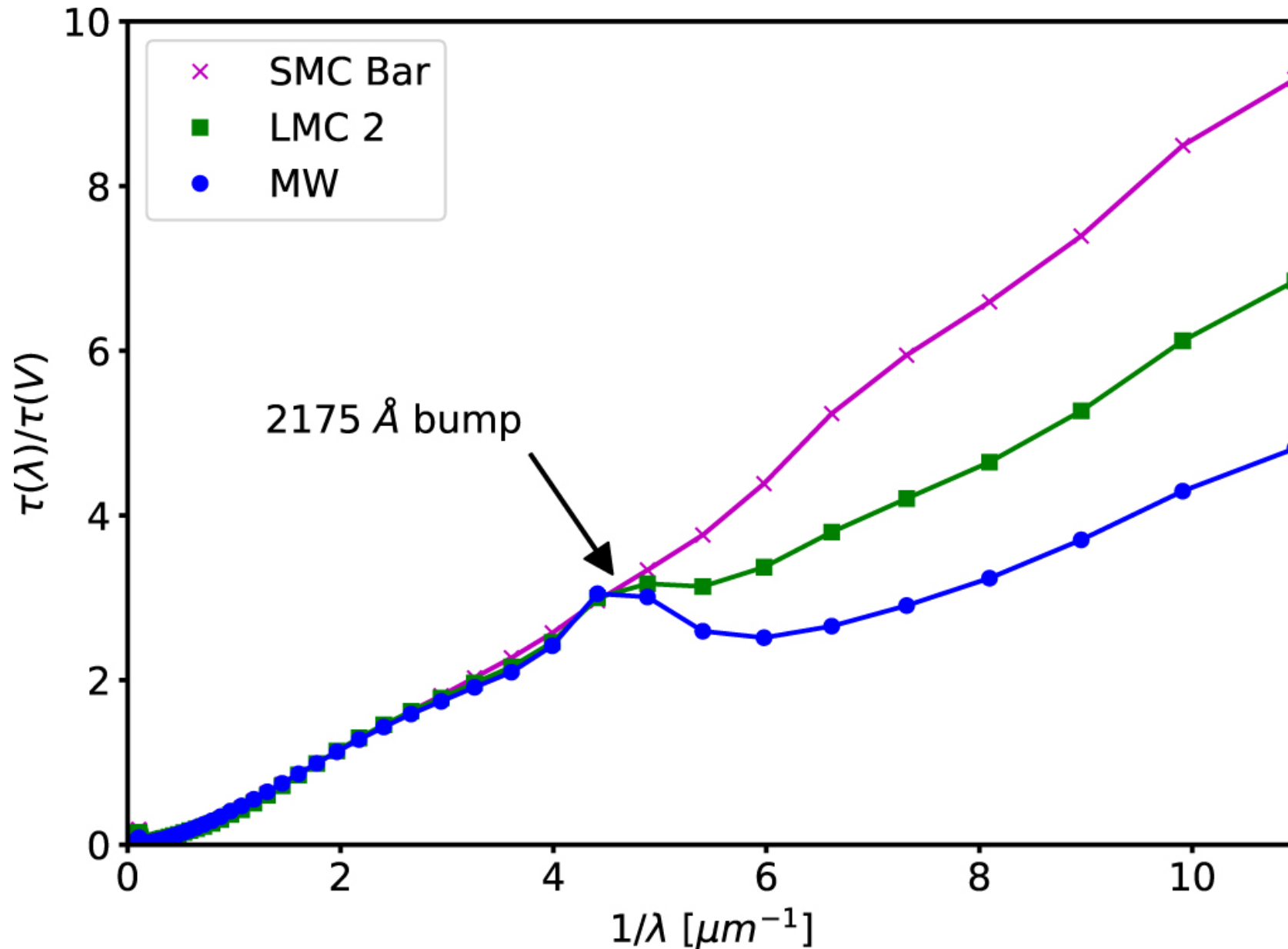
Figure 4. from DirtyGrid I: 3D Dust Radiative Transfer Modeling of Spectral Energy Distributions of Dusty Stellar Populations null 2018 APJS 236 32 doi:10.3847/1538-4365/aabf41 https://dx.doi.org/10.3847/1538-4365/aabf41 © 2018. The American Astronomical Society. All rights reserved.
