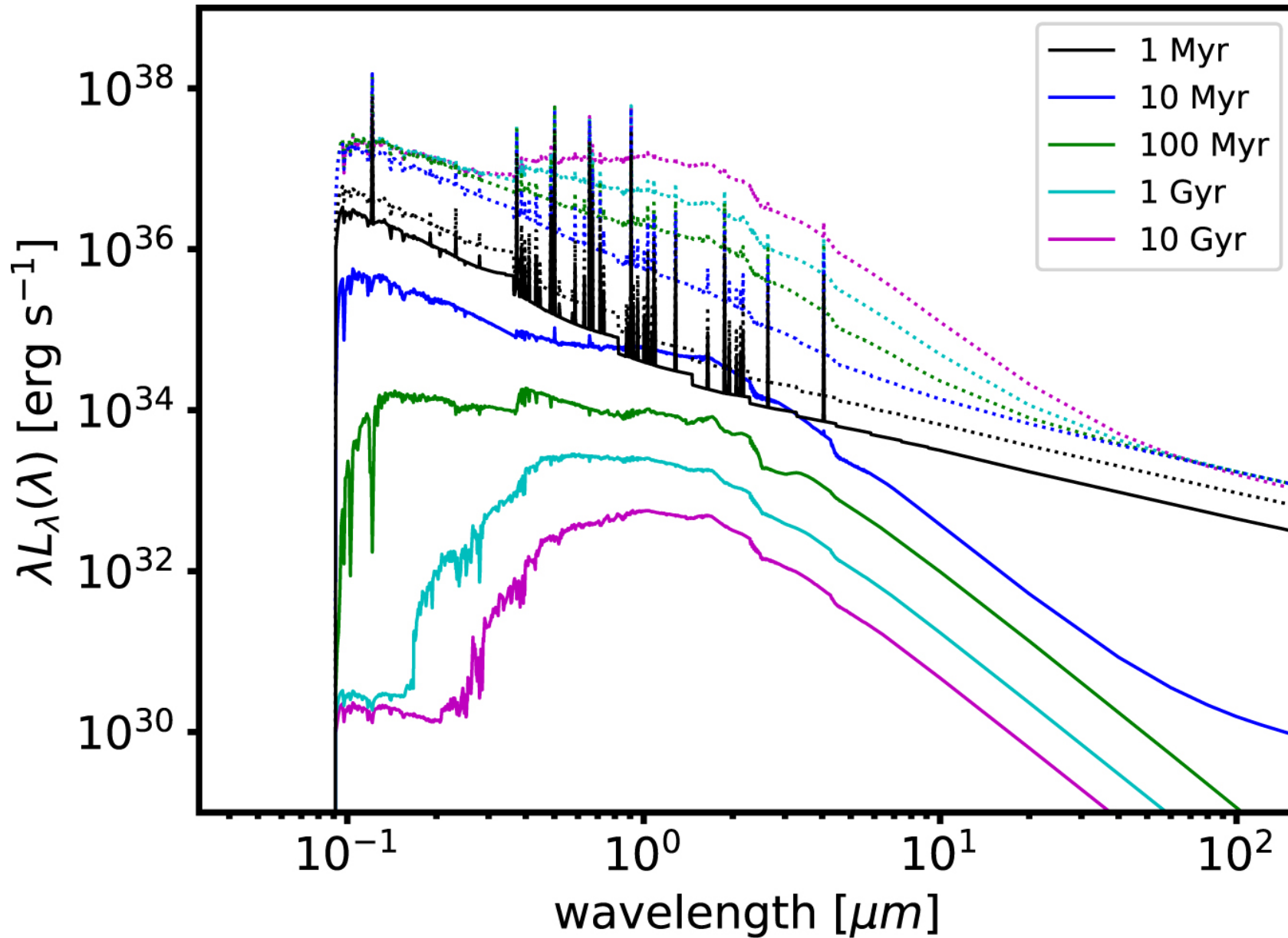
Figure 3. from DirtyGrid I: 3D Dust Radiative Transfer Modeling of Spectral Energy Distributions of Dusty Stellar Populations null 2018 APJS 236 32 doi:10.3847/1538-4365/aabf41 https://dx.doi.org/10.3847/1538-4365/aabf41 © 2018. The American Astronomical Society. All rights reserved.
