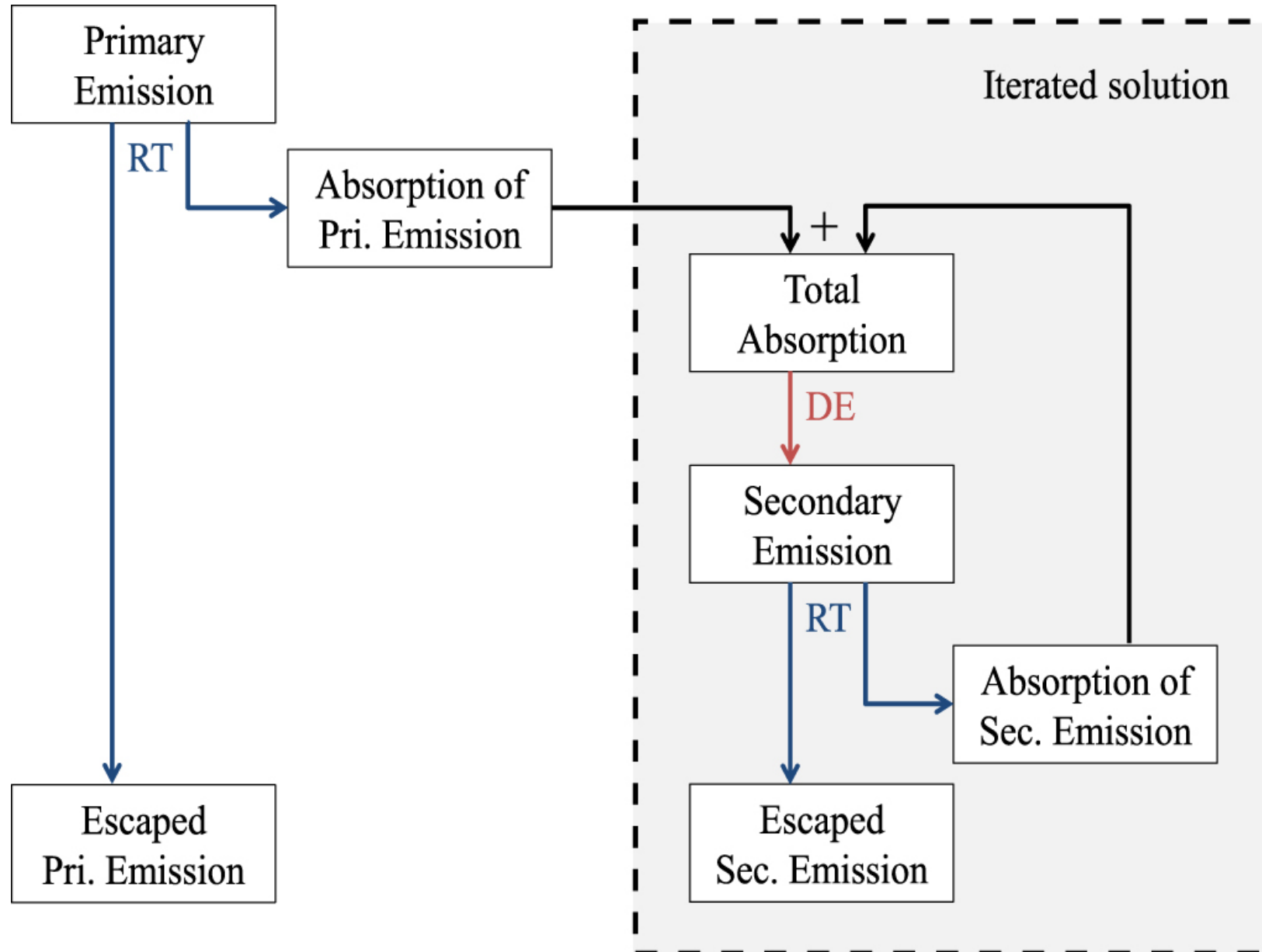
Figure 2. from DirtyGrid I: 3D Dust Radiative Transfer Modeling of Spectral Energy Distributions of Dusty Stellar Populations null 2018 APJS 236 32 doi:10.3847/1538-4365/aabf41 https://dx.doi.org/10.3847/1538-4365/aabf41 © 2018. The American Astronomical Society. All rights reserved.
