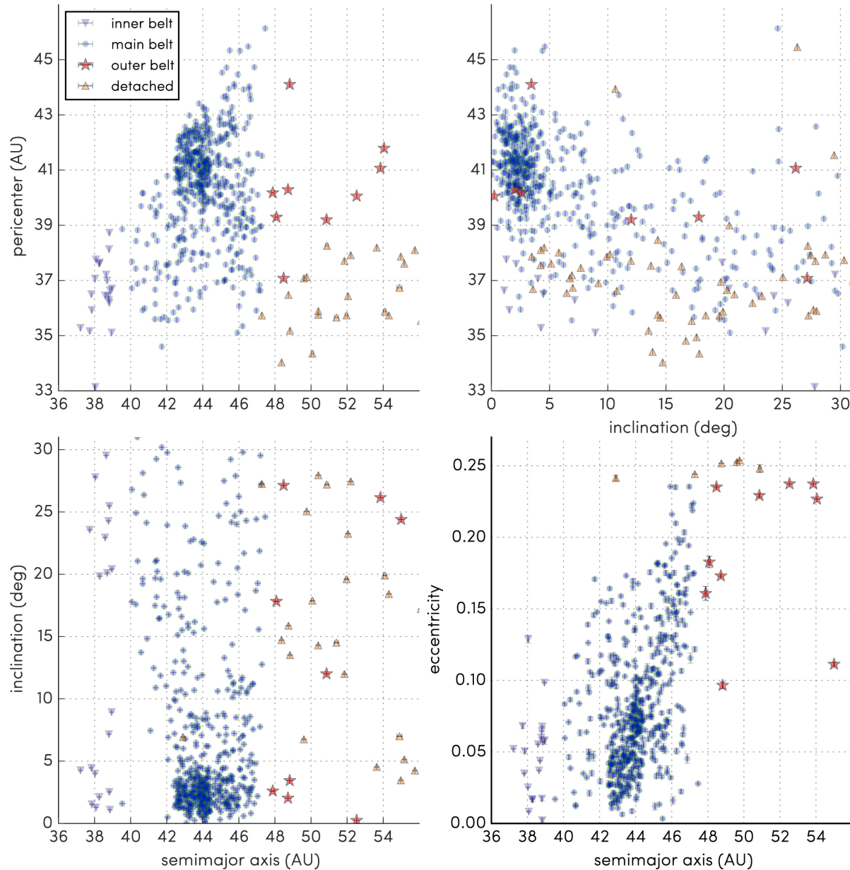
Figure 5. from OSSOS. VII. 800+ Trans-Neptunian Objects—The Complete Data Release null 2018 APJS 236 18 doi:10.3847/1538-4365/aab77a https://dx.doi.org/10.3847/1538-4365/aab77a © 2018. The American Astronomical Society. All rights reserved.
