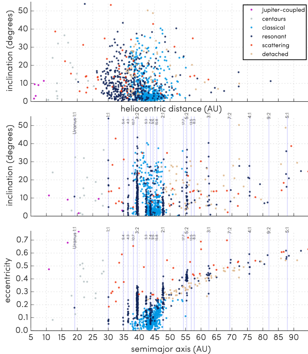
Figure 4. from OSSOS. VII. 800+ Trans-Neptunian Objects—The Complete Data Release null 2018 APJS 236 18 doi:10.3847/1538-4365/aab77a https://dx.doi.org/10.3847/1538-4365/aab77a © 2018. The American Astronomical Society. All rights reserved.
