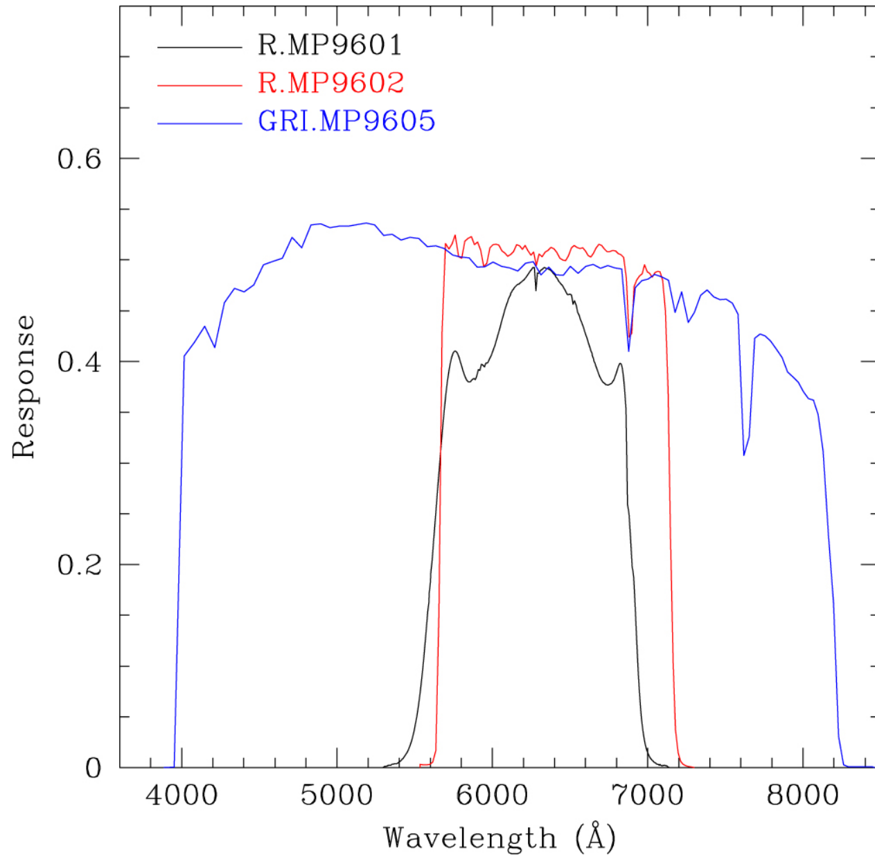
Figure 3. from OSSOS. VII. 800+ Trans-Neptunian Objects—The Complete Data Release null 2018 APJS 236 18 doi:10.3847/1538-4365/aab77a https://dx.doi.org/10.3847/1538-4365/aab77a © 2018. The American Astronomical Society. All rights reserved.
