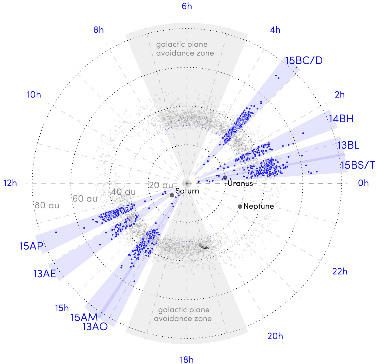
Figure 1. from OSSOS. VII. 800+ Trans-Neptunian Objects—The Complete Data Release null 2018 APJS 236 18 doi:10.3847/1538-4365/aab77a https://dx.doi.org/10.3847/1538-4365/aab77a © 2018. The American Astronomical Society. All rights reserved.
