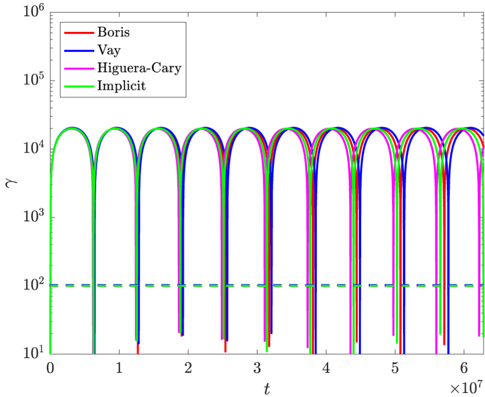
Figure 9. from A Comprehensive Comparison of Relativistic Particle Integrators null 2018 APJS 235 21 doi:10.3847/1538-4365/aab114 https://dx.doi.org/10.3847/1538-4365/aab114 © 2018. The American Astronomical Society. All rights reserved.
