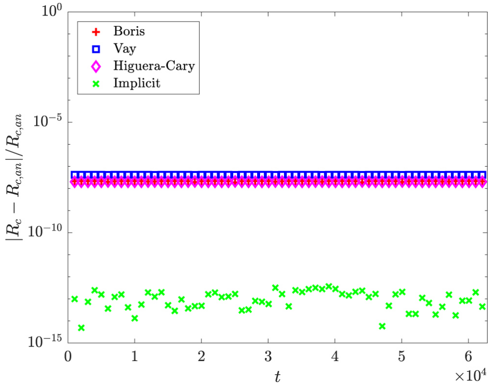
Figure 8. from A Comprehensive Comparison of Relativistic Particle Integrators null 2018 APJS 235 21 doi:10.3847/1538-4365/aab114 https://dx.doi.org/10.3847/1538-4365/aab114 © 2018. The American Astronomical Society. All rights reserved.
